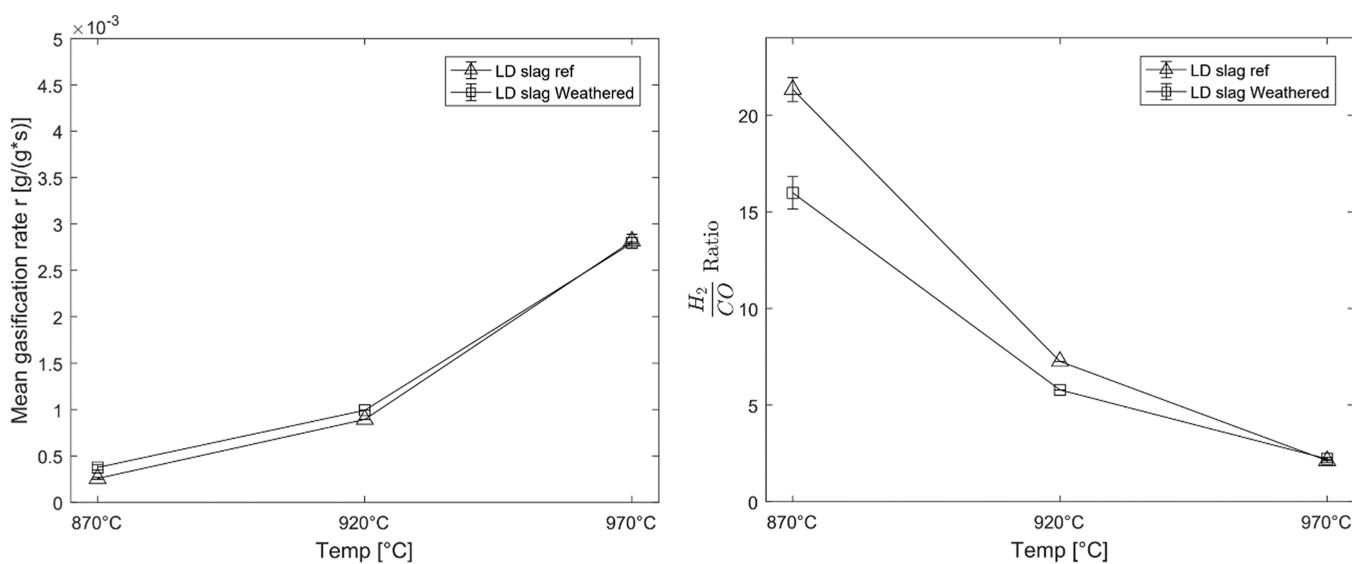
Figure 9. Left: mean gasification rate (mean taken from 0.3 < X C < 0.7) for LD slag that has been weathered compared to a reference sample of LD slag at different temperatures. Right: mean H 2 /CO ratio taken from 0.3 < X C < 0.7 with solid fuel for weathered LD slag compared to a reference sample of LD slag at different temperatures.
