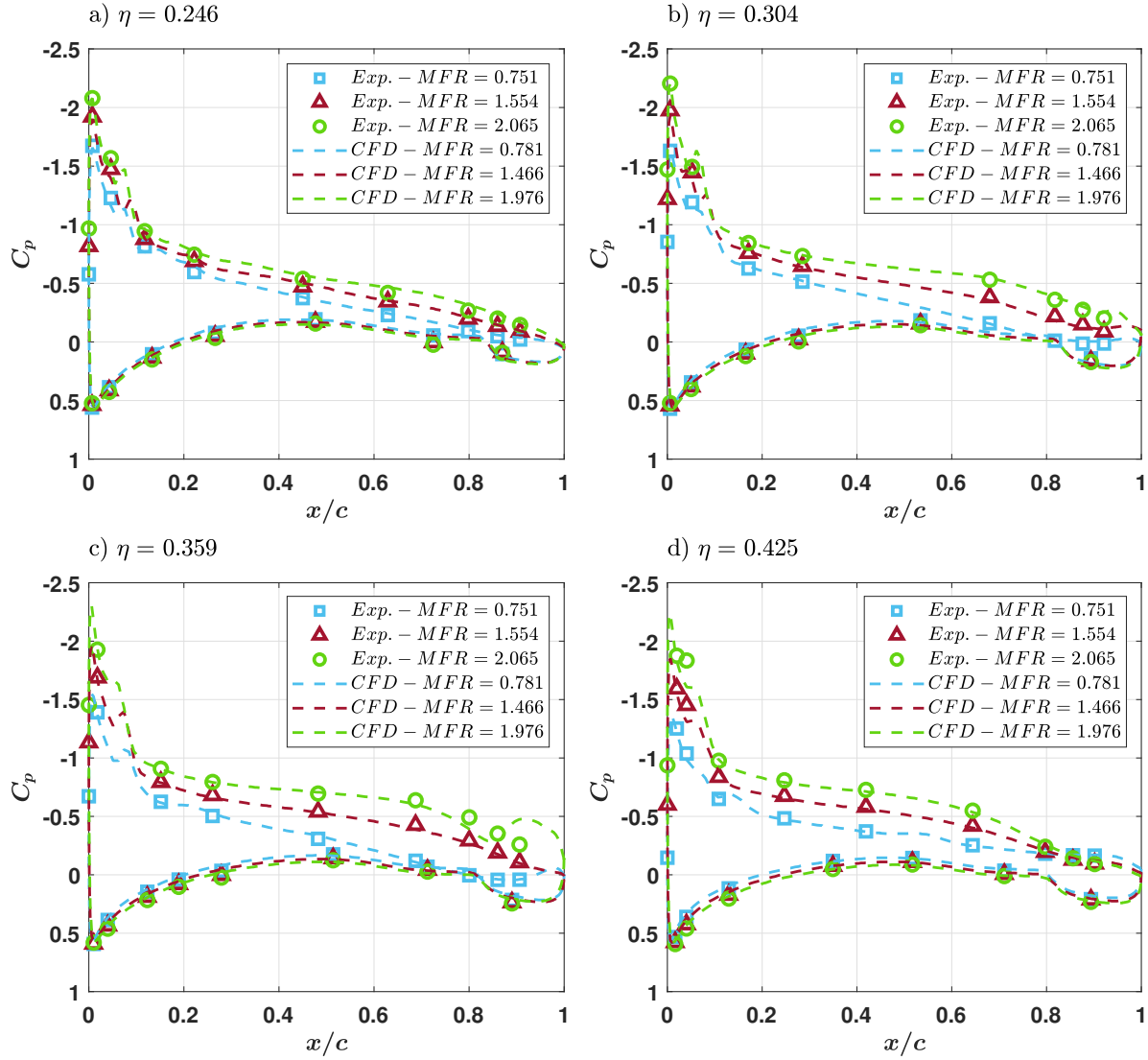
Fig. 11 Pressure distributions for AoA = 4^\circ . The experimental results are compared with CFD data for similar MFRs.
