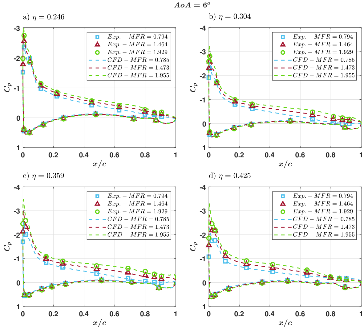
Fig. 12 Pressure distributions for AoA = 6^\circ . The experimental results are compared with CFD data for similar MFRs.
