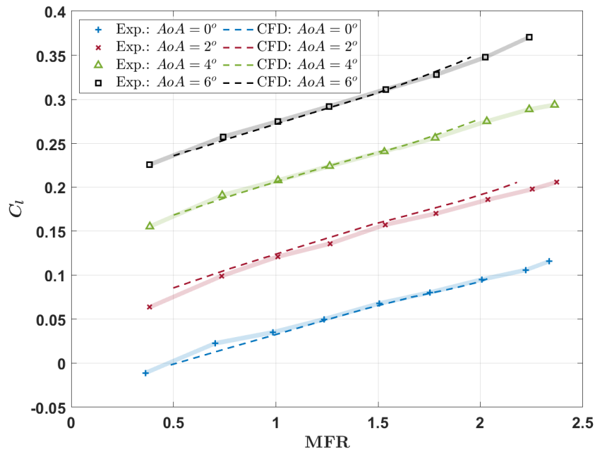
Fig. 8 The effect of the engine MFR on the aircraft C_l . The experimental results are compared to CFD data. The uncertainty of the measurements is represented by the shaded areas.
