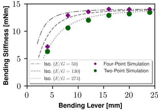
Figure 2.9: Results from two-point and four-point bending stiffness simulations for different bending levers for 200 g/m 2 paperboard composed entirely of CTMP. The dashed line is a prediction based on the experimental tensile stiffness of the sheet using a Timoshenko beam representation of the paper sheet.
