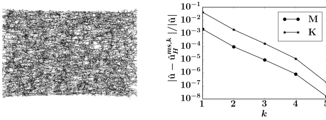
Figure 4.3: The solution of the two-dimensional equilibrium tensile simulation, and the k -convergence results for the LOD approximation.
