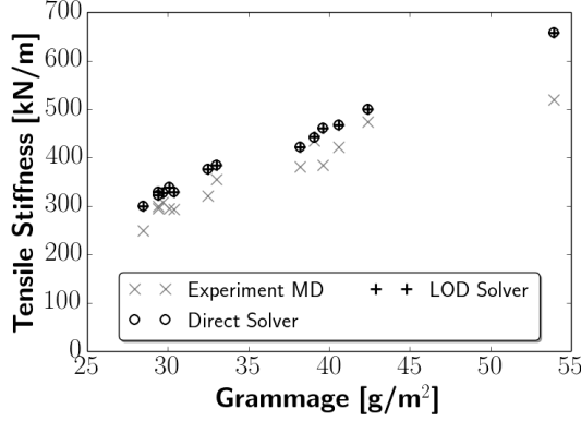
Figure 4.4: Tensile stiffness simulations using the LOD method.
