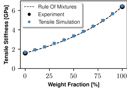
Figure 2.7: Tensile stiffness for different weight distributions in various 200 g/m 2 three-ply paperboard. The black circular markers are experimental measurements, the colored cross markers are simulated results, and the dashed lines are the rule of mixtures based on the experimental tensile stiffness in [45] of sheets made from one pulp.
