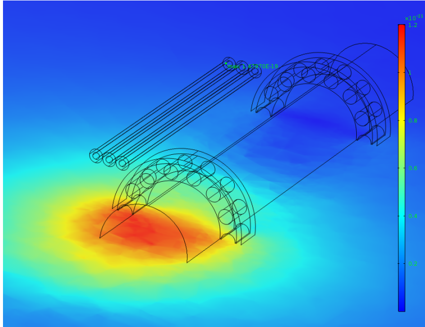
Figure 4.13: Magnetic field distribution near the shaft
