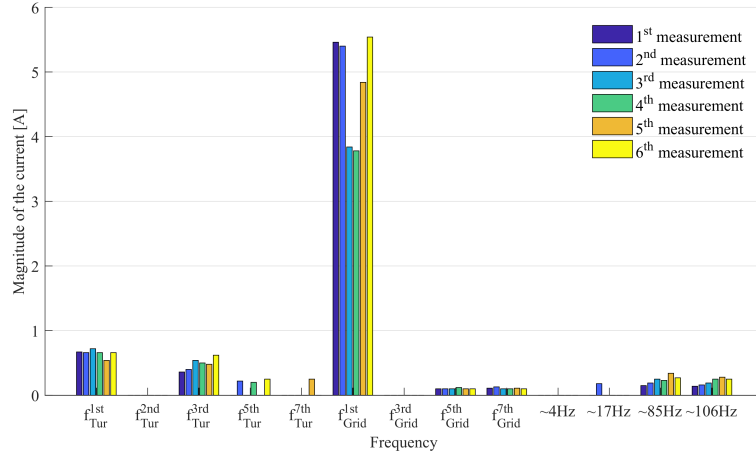
(a) Shaft current
