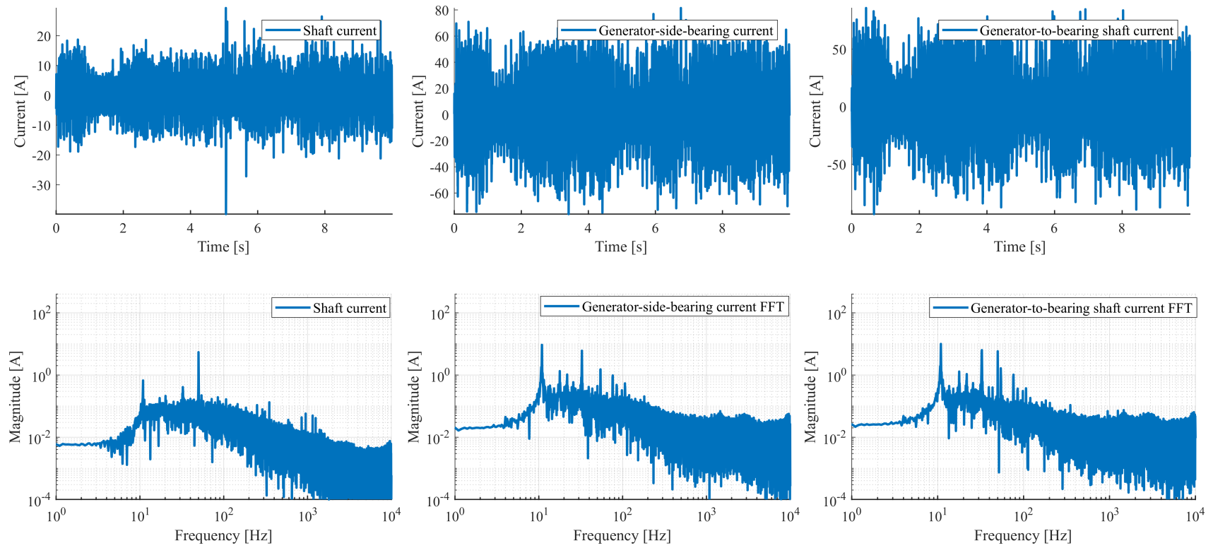
Figure 4.9: The waveforms and the single-sided amplitude spectra of the currents in the shaft and the current through the bearing near the generator for the first measurement performed on November 15 th 2017
