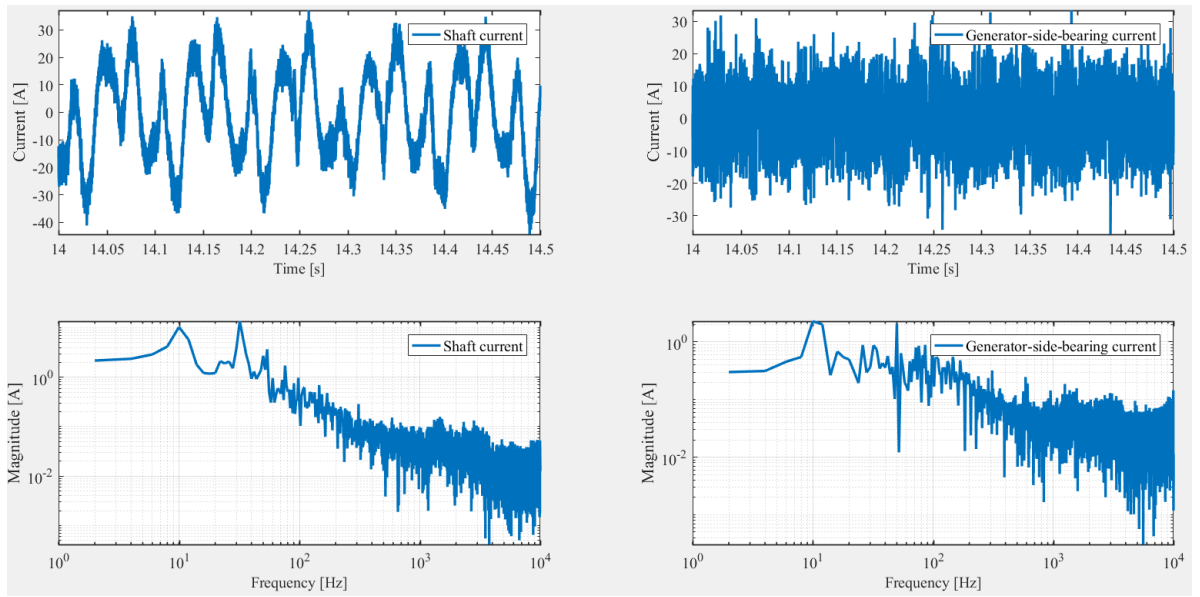
Figure A.7: (derived with applying KCL) Shaft current and generator-side-bearing current waveforms and single-sided amplitude spectrum for the 4 th measurement (drift3-C10V, 14 < t < 18) performed at the Big Glenn site on April 11 th 2017.
