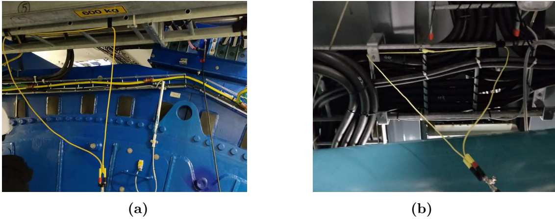
Figure 3.4: The voltage measurement loops at Big Glenn site (a) near the generator (b) above the shaft
