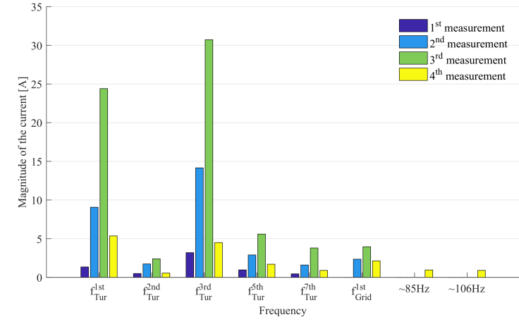
(b) Generator-side bearing current
