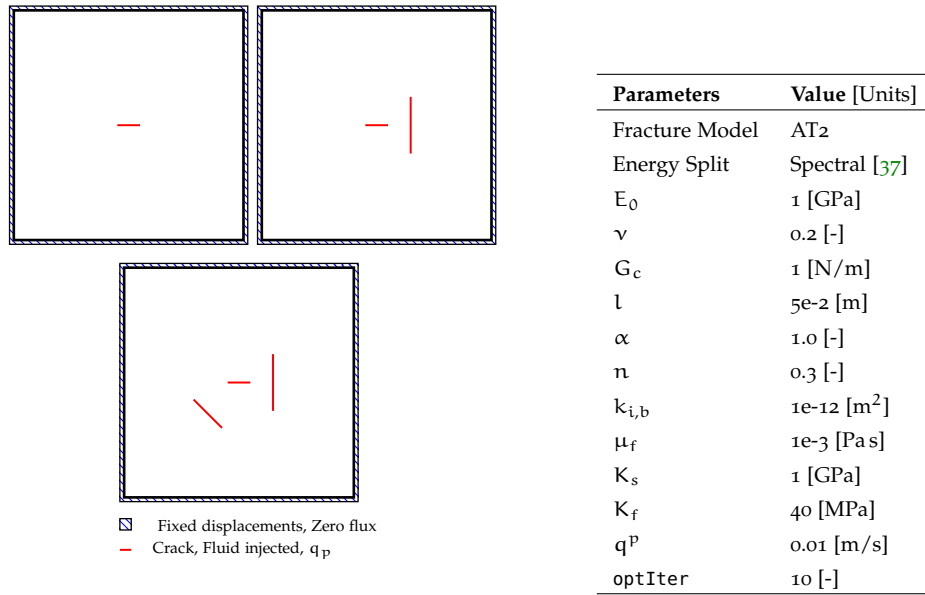
Figure 5.1: Specimen with single, double and triple initial fractures (SNF, DNF, TNF)
