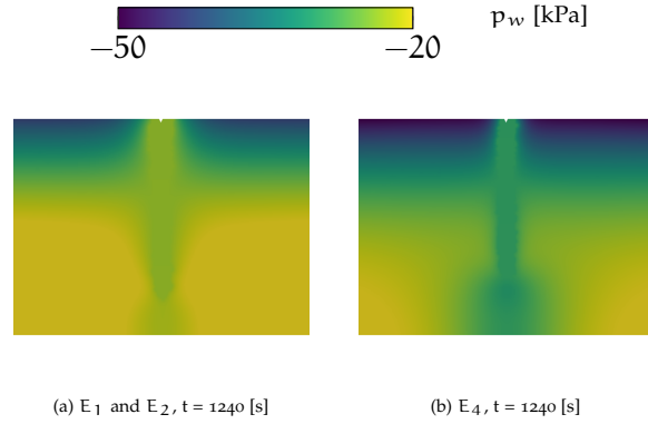
Figure 6.5: Figures (a-b) present the distribution of the water pressure with energy functionals E_1 , E_2 and E_4 during the analysis of the small notched specimen. The effective permeability K_{eff} (6.19) is enhanced with a fracture permeability K_f (6.17).
