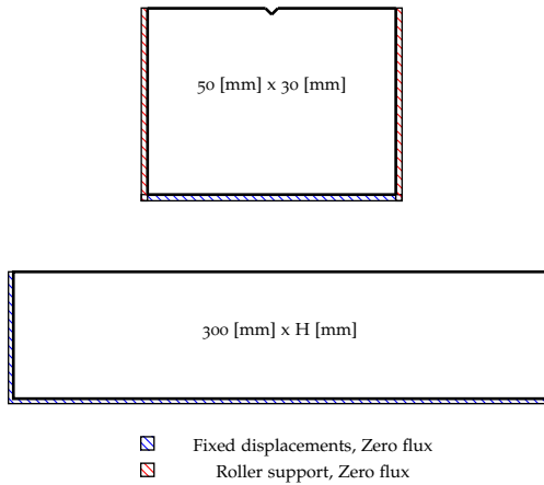
Figure 6.1: Soil desiccation cracking specimens
