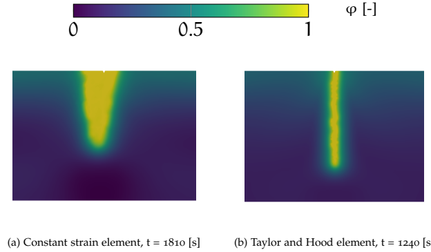
Figure A.3: Figures (a-b) present the distribution of the phase-field variable pertinent to the energy functional E_4 . The sub-figures correspond to the 3-noded constant strain element and the 6-noded Taylor and Hood element, respectively.
