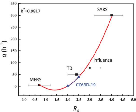
Fig. 2 The fitted curve between the quantity q and basic reproductive number ( R_0 ) (without
