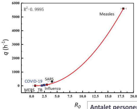
Fig. 1 The fitted curve between the quantity q and basic reproductive number ( R_0 ) (with
