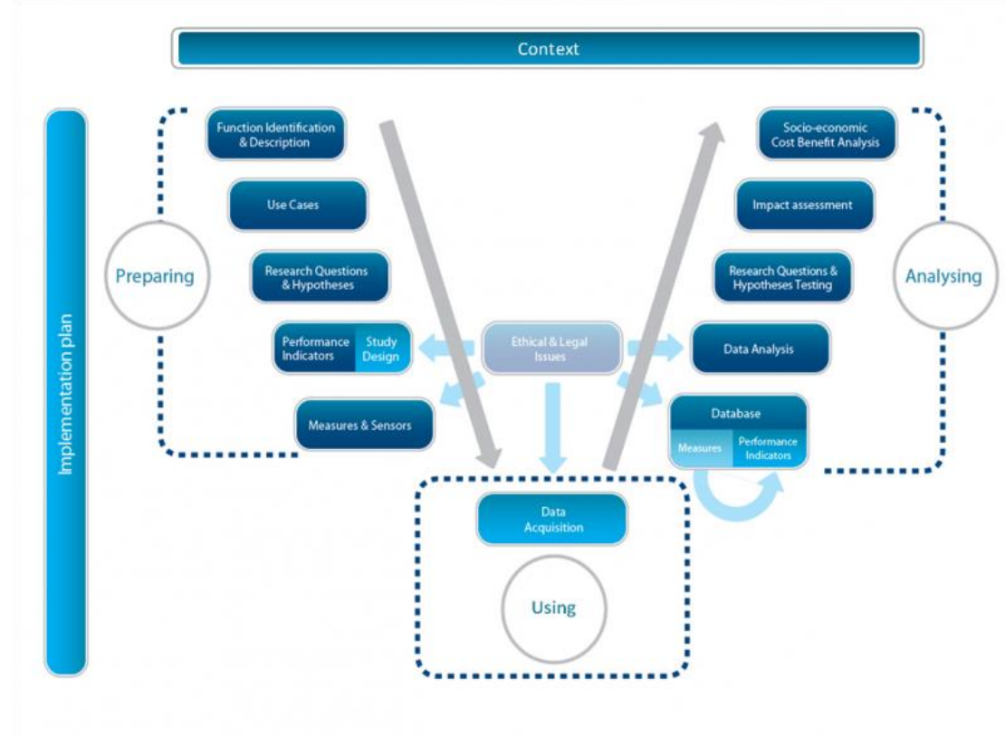
Figure 7. FESTA V-diagram
