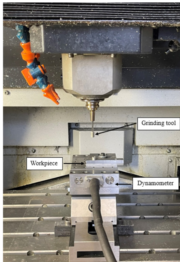
Fig. 2. Experimental setup
