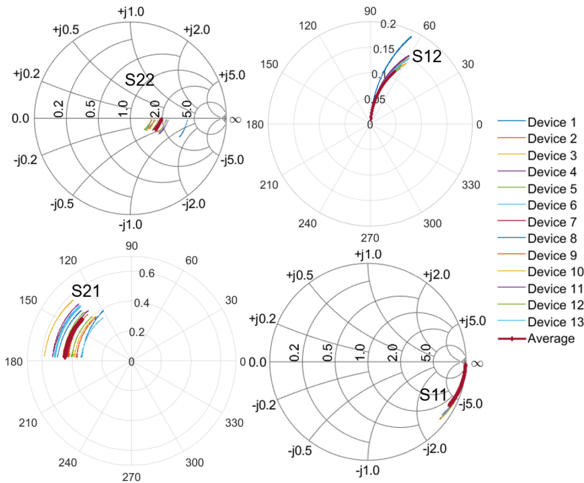
FIGURE 1. S-parameters measured between 1 GHz and 20 GHz at optimum gate bias and V_D = 1.2 V for a set of thirteen different GFETs (#1 – 13) fabricated on the same chip. The total width of the GFET is 30 \mu\text{m} .
