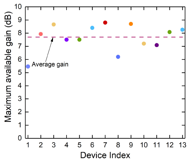
FIGURE 2. Calculated maximum available gain (MAG) at 10.5 GHz for a set of thirteen different GFETs (#1 – 13) fabricated on the same chip.
