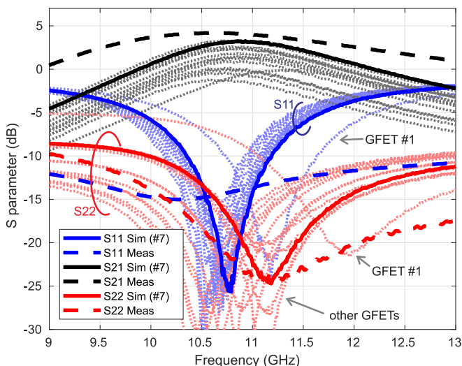
FIGURE 7. Integrated GFET amplifier performance at room temperature. Measured and simulated S -parameters of the complete circuit. Grey lines indicate simulations with other GFETs as shown in Fig. 1. The transistor was biased at V_{GS} = 0.5 \text{ V} and V_{DS} = -1.3 \text{ V} .
