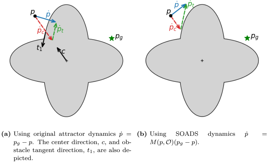
Figure 3.2: The velocity vector \dot{p} and the vectors \dot{p}_c and \dot{p}_t defined as the decomposition along the center direction c and the obstacle tangent direction t_1 , respectively.
