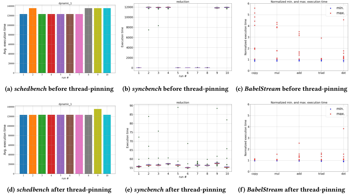
Figure 4: Lower variability of execution time ( \mu s) after thread-pinning in schedbench (first column) when using 16 threads, and in syncbench (second column) and in BabelStream (third column) when using 128 threads on Dardel.
