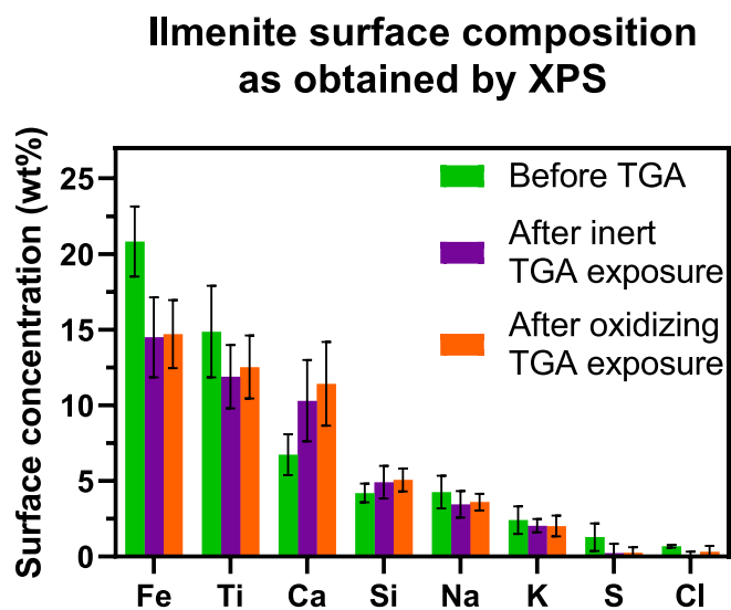
Fig. 11. Summary of the surface composition of ilmenite particles obtained by XPS for samples before TGA experiment and after TGA experiments in both inert and oxidizing atmospheres at 1000 °C for 10 h.
