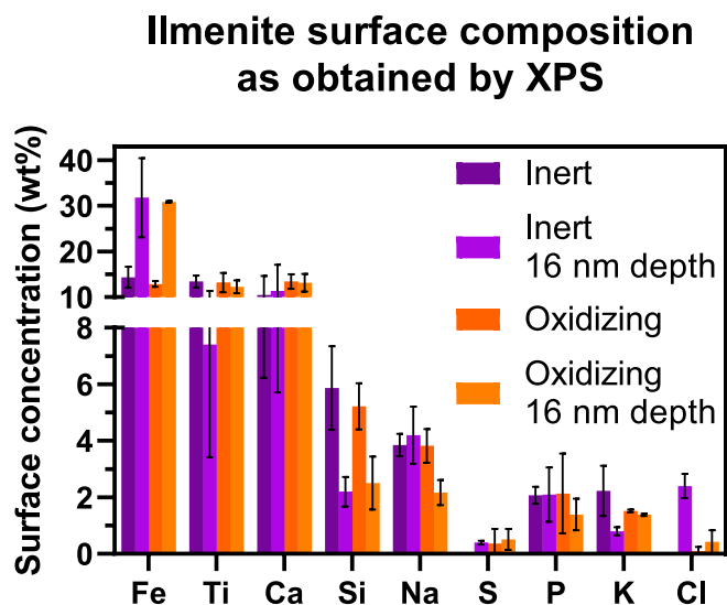
Fig. 12. Surface composition of ilmenite particles obtained by XPS. Composition is obtained at 16 nm depth generated by sputtering, and compared with the outermost surface composition. Samples obtained after TGA experiments in inert and oxidizing atmospheres at 1000 °C for 10 h.
