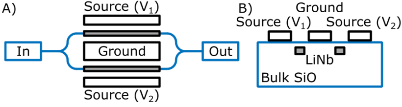
Figure 2.8: A top (A) and side (B) view of an idealized, chip based MZM. Here, an optical input is split into two arms - each of which produces phase modulation via the electro-optic effect. This is done by generating an electric field between the ground and source which thereby modulates the Lithium Niobate (LiNb). Not pictured here is the mechanism required for fixing V_1(t) = -V_2(t) for pure amplitude modulation.
