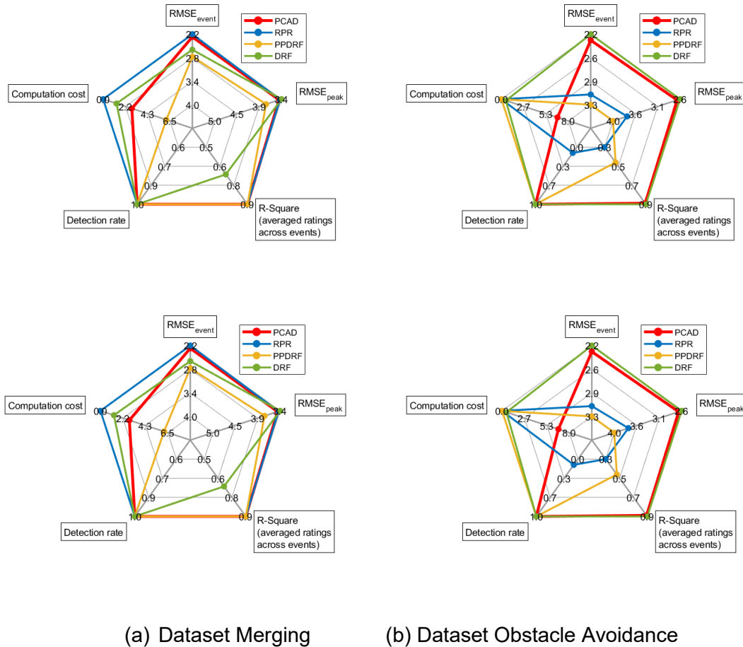
Figure 10. Radar charts of performance indicators comparing the PCAD model with three existing models for two datasets: the farther from the centre, the better the performance.
