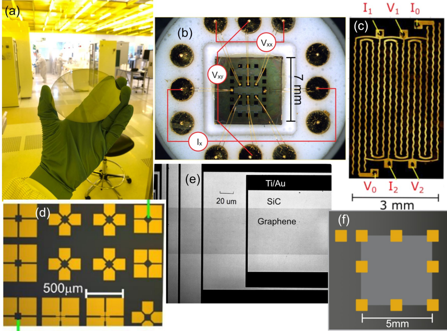
Figure 1.4: Collage of different types of devices fabricated in this thesis using epitaxially grown graphene over 4H-SiC. (a) Example of epigraphene grown on 4-inch SiC substrate. (b) Hall bars of the size \sim 5 \text{ mm} \times 2 \text{ mm} were used for stability analysis of molecular dopants. (c) Quantum Hall Array (QHA) consisting of 236 Hall elements, with a footprint of 3 \text{ mm} \times 6 \text{ mm} . (d) Large area fabrication of Hall sensors. (e) Transfer length geometry fabricated to analyze the contact resistance of scalable edge contacts (f) Ultraviolet (UV) detector spanning nearly 5 \text{ mm} \times 5 \text{ mm} area over a 7 \text{ mm} \times 7 \text{ mm} chip. (b) to (f) Device geometry ranges from a few micrometers to several millimeters, indicating true scalability of growth as well as fabrication methods.
