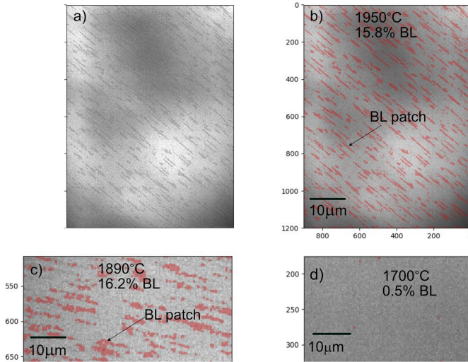
Figure 4.7: (a) Transmission mode optical microscopy image, used to quantify the graphene BL coverage percentage. Digital image processing such as image saturation and gamma corrections are adjusted to enhance the contrast between ML and BL graphene. In images (b) - (c) red areas are the BL graphene regions highlighted by the image processing Python script. It also shows the progress in the growth quality after the cyclic optimization procedure. Here temperature is used as one of the parameters to suppress BL growth.
