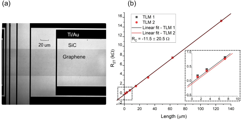
Figure 5.6: Analysis of contacts to epigrahene using the Transfer Length Method (TLM). (a) Optical microscopy image in transmission mode illustrating the fabricated edge-contacted TLM device. (b) Example of TLM data for two devices with 64 μm wide epigrahene channels measured at T = 300 K. It is important to note that the resulting fit yields a negative (unphysical) R_C , approaching zero, with an uncertainty of \pm 20.5 \Omega . Inset: a closer examination of the TLM data for L < 10 \mu\text{m} .
