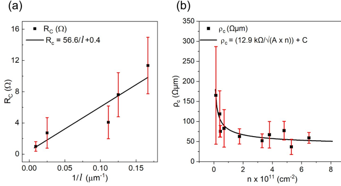
Figure 5.8: Characterization of the metal-graphene interface was conducted using the three-probe configuration in the quantum Hall regime ( T = 4 \text{ K} , B = 5 \text{ T} ). (a) R_C ( \Omega ) was plotted against the inverse perimeter length for five devices situated on the same chip. The linear fit resulted in a resistance R_C(l) = 56.6/l + 0.4 \text{ } \Omega . (b) \rho_C was plotted against carrier concentration. The solid line represents a fit to \rho_C = h/(2e^2 \sqrt{n_{eff}}) + C , where n_{eff} = A \times n . Here, n_{eff} signifies an effective carrier density at the carrier injection points (hot spots). The fits returned the values A = 19.7 and C = 34.5 \text{ } \Omega\mu\text{m} . The error bars represent one standard deviation from the mean value.
