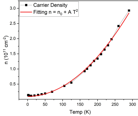
Figure 6.4: The temperature dependence of the effective carrier density n_e , obtained from [17], is shown in black. The red data points represent the fit using the model for disorder-induced temperature-dependent transport from [22], enabling the extraction of the disorder strength s .
