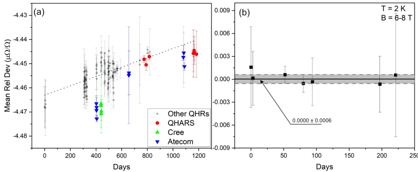
Figure 7.10: (a) Precision Cryogenic Current Comparator (CCC) measurements of a 100\ \Omega resistance standard compared against various Quantum Hall Resistance Standard (QHRS). These comparison measurements were conducted against different graphene QHRs ('Other QHR'), Quantum Hall Array Resistance standards (QHARSs), as well as the Cree and Atecom samples discussed in this study. The slope of the mean relative deviation between the 100\ \Omega standard and the various QHRs over a three-year period suggests that the drift in the 100\ \Omega resistor amounts to approximately 2\ \text{n}\Omega/\Omega per 100 days. The error bars represent one standard deviation. (b) Shows the precision measurements directly comparing graphene quantum Hall arrays stored in a desiccant/oxygen absorber environment. The grey-shaded area represents one standard deviation from the weighted mean (black line) of all data points. The mean relative deviation among the QHARSs is within 0.03\ \text{n}\Omega/\Omega with an uncertainty of 0.6\ \text{n}\Omega/\Omega .
