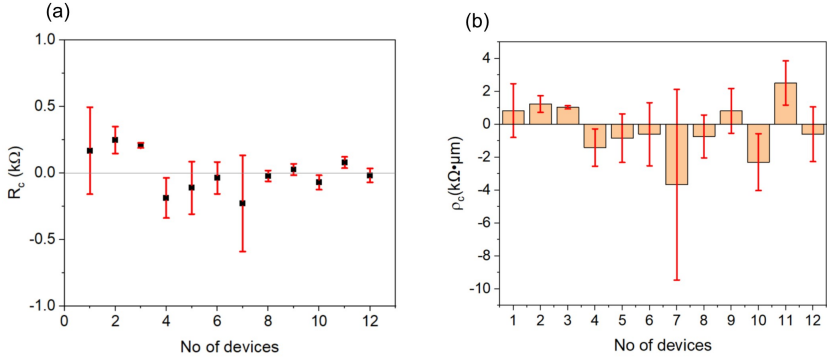
Figure 5.7: TLM assessments were performed on the 12 epigrahene device structures patterned across five epigrahene chips. (a) The R_C values (kΩ) correspond to the 12 devices, where 7 of them yield negative (non-physical) results. (b) The computed values of \rho_C indicate a substantial diversity in resistance, with a mean of -500.74 \Omega\mu\text{m} and a standard deviation of \pm 1770.24 \Omega\mu\text{m} , which are not physically viable.
