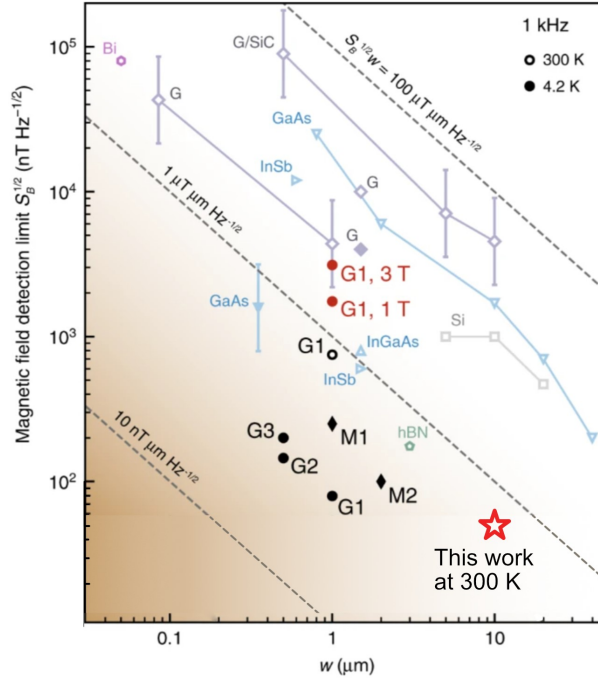
Figure 6.1: Comparison of magnetic field detection limit [64]. Epigraphene hall sensors fabricated in this work outperform the best-reported Hall sensors in the literature.
