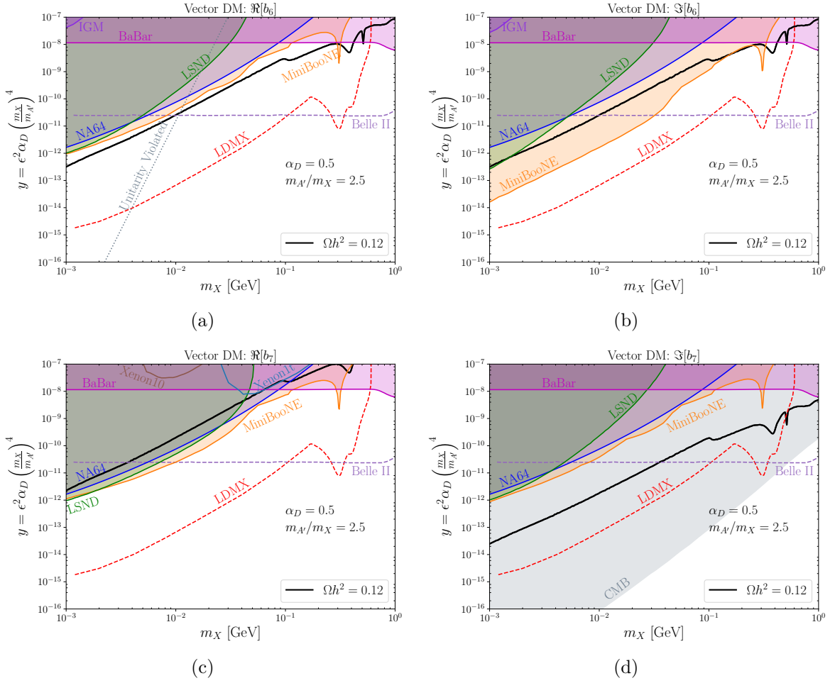
Figure 5. Same as figure 4, now for the mass ratio m_{A'} = 2.5 m_\chi . For this choice of parameters, the \text{Re}[b_6] model predicts the current DM relic abundance, is compatible with observations, and is within reach at LDMX in the mass range between about 10 MeV and 300 MeV.
