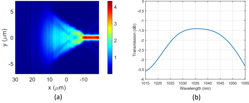
Figure 4.11: 3D-FDTD simulation an apodized focusing grating coupler (channel 3: 1039 nm) with a bottom DBR. (a) Electric field profile of the grating in the xy plan. (b) Coupling efficiency of the device.
