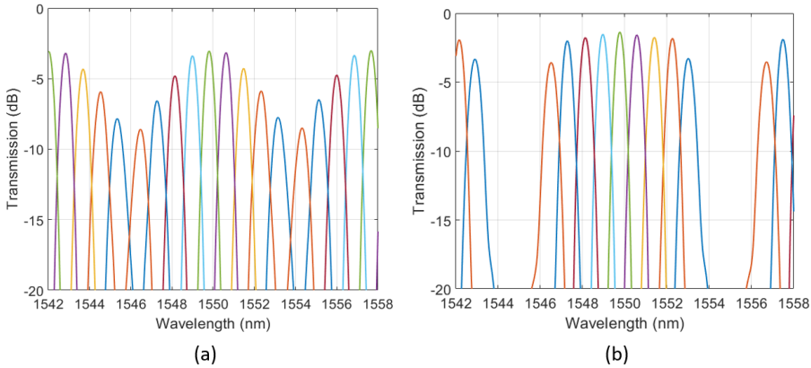
Figure 6.4: Simulations of AWGs with FSR of (a) 8 nm and (b) 10 nm.
