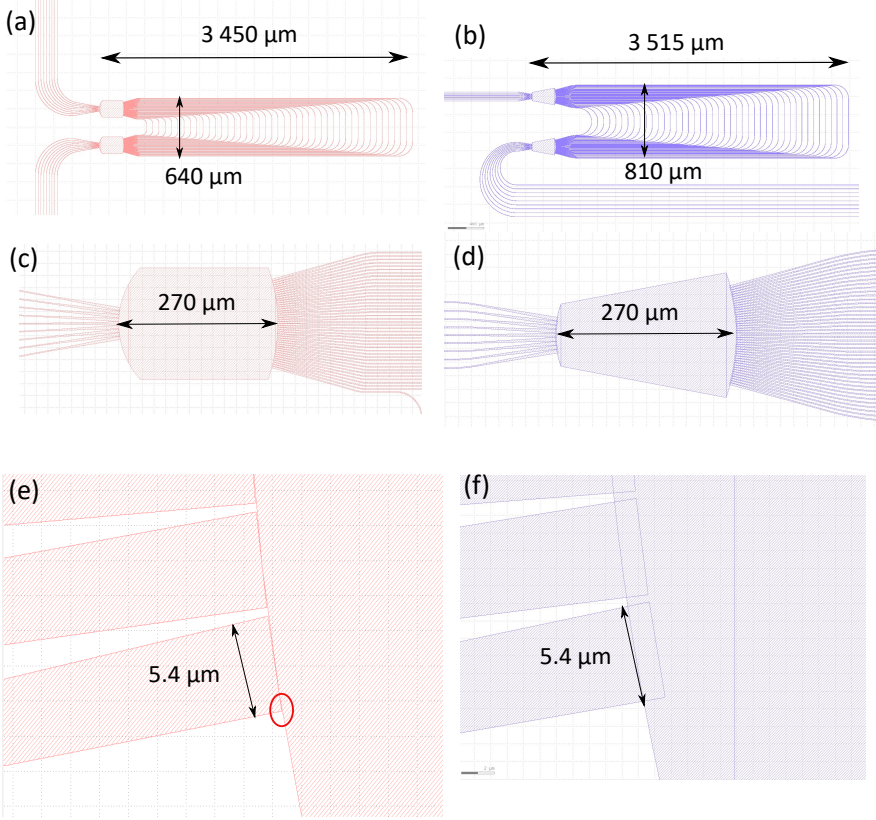
Figure 6.8: Comparison between the KLayouts of the (a), (c) and (e) AWG generated by the WDM PHASAR software and the (b), (d) and (f) AWG coded in Python. (a) and (b) Overall view of both devices. (c) and (d) Zoom at the first FPR. (e) and (f) Zoom at the receiver waveguides - FPR section. The red circle in (e) highlights a 26 nm wide gap between the taper and the FPR.
