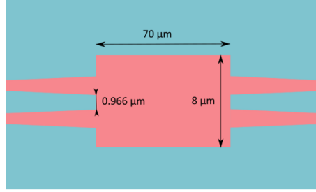
Figure 3.5: Illustration of the designed 2 x 2 MMI.
