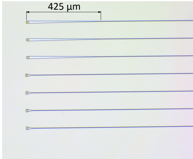
Figure 4.13: Manufactured apodized straight and focusing grating couplers
