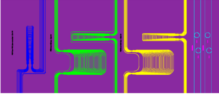
Figure 6.5: Mask layout of the chip. The distance between the FPRs for the small AWGs is 400\ \mu\text{m} and is 4000\ \mu\text{m} for the wide AWGs.
