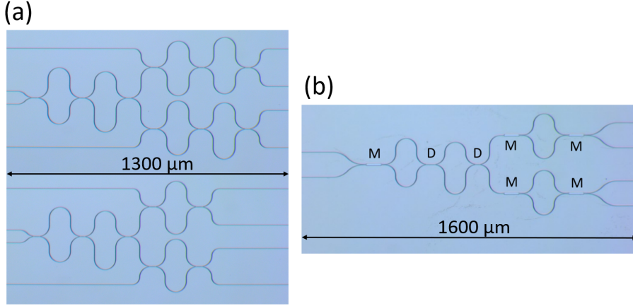
Figure 3.16: (a) Manufactured cascaded MZIs based on DCs exclusively. The bottom device is a 2 nd -to-1 st order filter and the top device is a 2 nd -to-2 nd order filter. (b) Manufactured cascaded MZIs based on DCs and MMIs. The 'M' and 'D' letters are for MMI and DC respectively.
