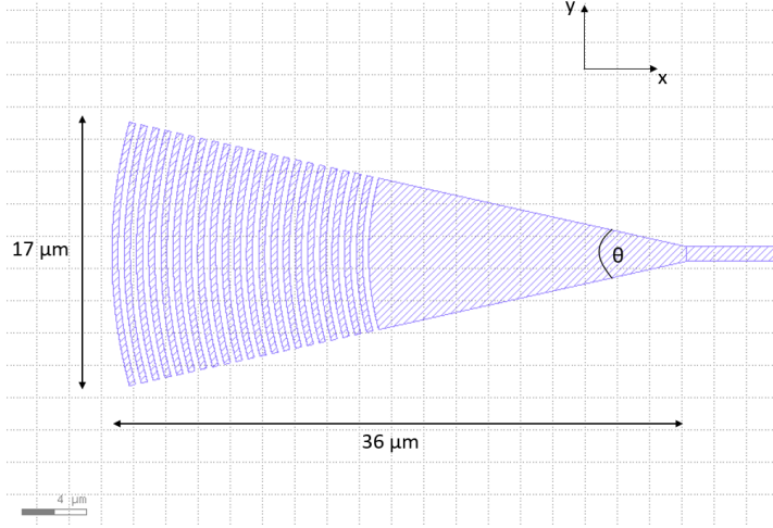
Figure 4.10: Designed focusing grating coupler in KLayout.
