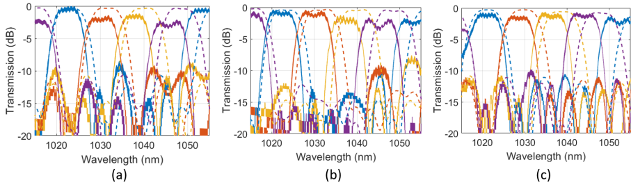
Figure 3.17: Simulation (dashed curves) and measurements (continuous curves) of the (a) 2 nd -to-1 st order MZI filter based on DCs, (b) 2 nd -to-2 nd order MZI filter based on DCs, (c) cascaded MZI based on DCs and MMIs.
