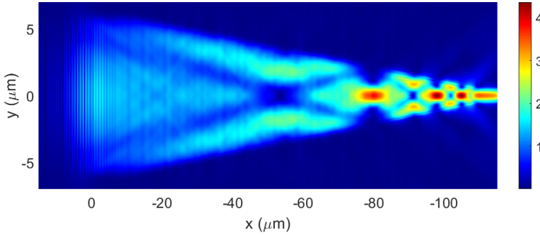
Figure 4.9: Electric field profile of a straight grating coupler with a 100\ \mu\text{m} -long linear taper
