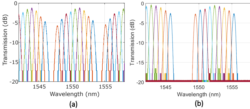
Figure 6.7: Characterization results of the AWGs. (a) DEMUX based on the 1500 nm x 200 nm waveguide with a designed FSR of 8nm. (b) DEMUX based on the 1000 nm x 200 nm waveguide with a designed FSR of 10 nm. The polarization state is TE.
