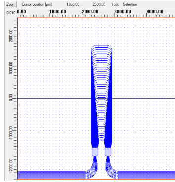
Figure 6.3: Device layout created from WDM PHASAR software.
