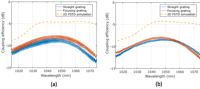
Figure 4.14: Measured coupling efficiencies of the apodized straight and focusing grating couplers for (a) channel No. 2 and (b) channel No. 3. 2D FDTD simulation of the corresponding grating coupler is also included.
