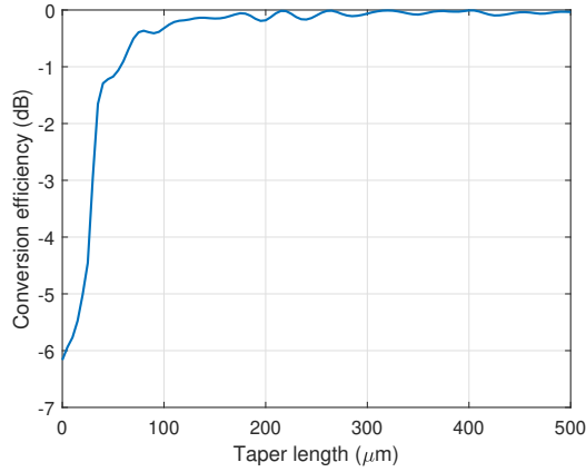
Figure 4.8: EME Simulation of the conversion efficiency of a linear taper. The slab-waveguide is 12\ \mu\text{m} wide and the output waveguide 0.9\ \mu\text{m} wide for a thickness of 160\ \text{nm} .
