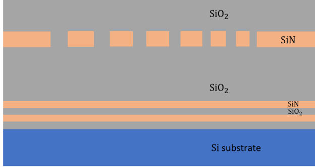
Figure 4.5: Schematic illustration of the apodized DBR-based grating coupler. The real device has 20 grating lines and 6 pairs of \text{SiO}_2/\text{SiN} bottom layers.
