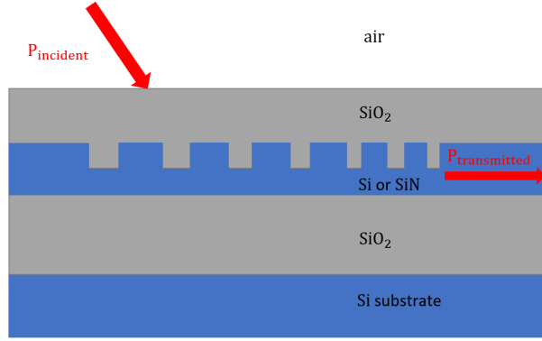
Figure 4.3: Illustration of an appodized grating coupler
