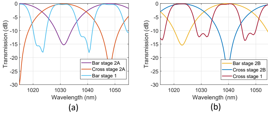
Figure 3.15: Simulation of (a) the upper arm MZI filter (Stage 2A) and (b) the lower arm MZI filter (Stage 2B)
