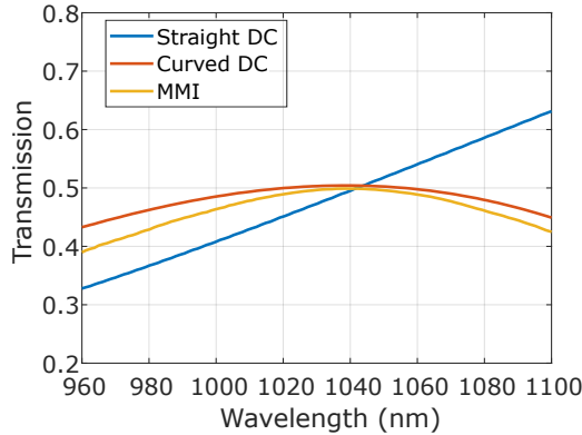
Figure 3.10: Comparison of the simulated (with varFDTD) cross output transmission of the straight, curved DC and MMI for the 50:50 splitting ratio.
