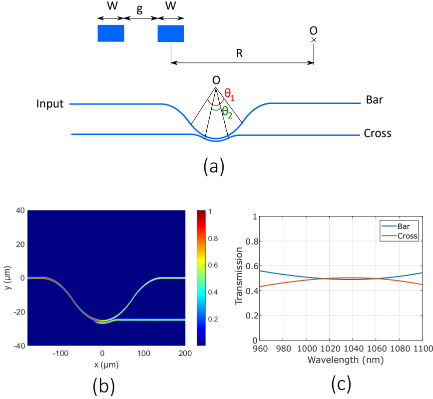
Figure 3.9: (a) Cross section of the curved DC with a scheme of the full device. Here, g = 340 \text{ nm} , R = 210 \text{ }\mu\text{m} , \theta_1 = 40^\circ and \theta_2 = 10.82^\circ . (b) Electric field profile of the curved DC. (c) varFDTD simulation of the transmission of the device for the 50:50 splitting ratio.
