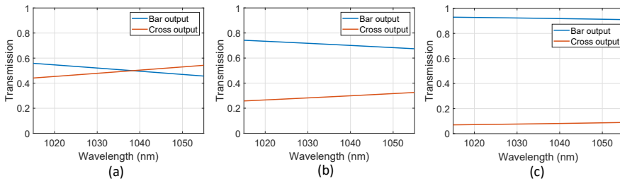
Figure 3.8: Transmission of the DC for K = (a) 0.5 (b) 0.29 (c) 0.08.
