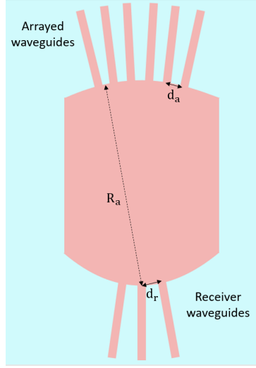
Figure 3.12: Scheme of the AWG star coupler
