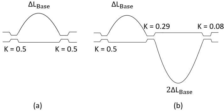
Figure 3.14: Schemes of first order (a) and second order (b) MZI filters. The K coefficients refer to the cross coupling coefficients of the directional couplers (or MMIs).
