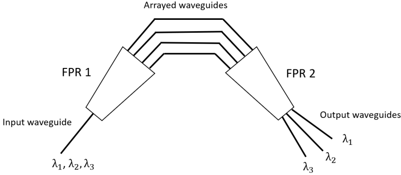
Figure 3.3: Illustration of an AWG
