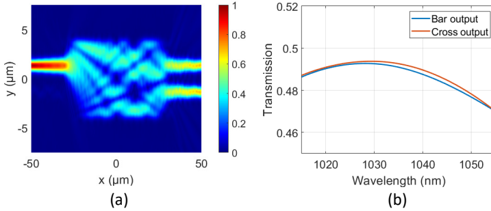
Figure 3.6: (a) varFDTD simulated power distribution of the MMI for the TE mode. (b) Transmission of the MMI. The 'Bar' and 'Cross' outputs are respectively the upper and lower outputs when the upper input is selected.
