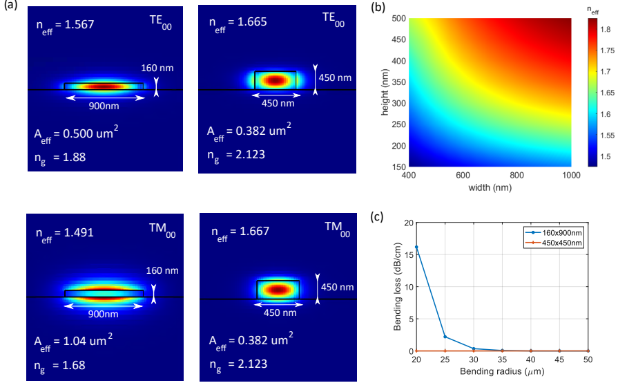
Figure 5.1: (a) Electric field of the TE 00 and TM 00 modes for the thin and thick waveguide. The FDE simulation results of the effective and group index ( n_{\text{eff}} and n_g respectively) and of the mode effective area ( A_{\text{eff}} ) are also presented. (b) n_{\text{eff}} for different waveguide dimensions. (c) Simulation of the bending loss for both waveguides.
