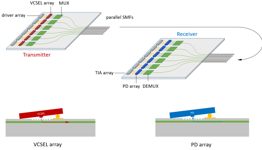
Figure 3.1: Short reach CWDM at 1060 nm. The light from the VCSEL array is coupled through grating couplers and guided to a multiplexer (MUX), a demultiplexer (DEMUX) and to an array of photodiodes (PD).
