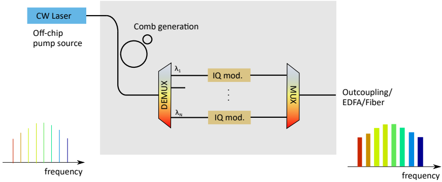
Figure 6.1: 1.55 \mu\text{m} interconnect: scheme of the multilayer chip.
