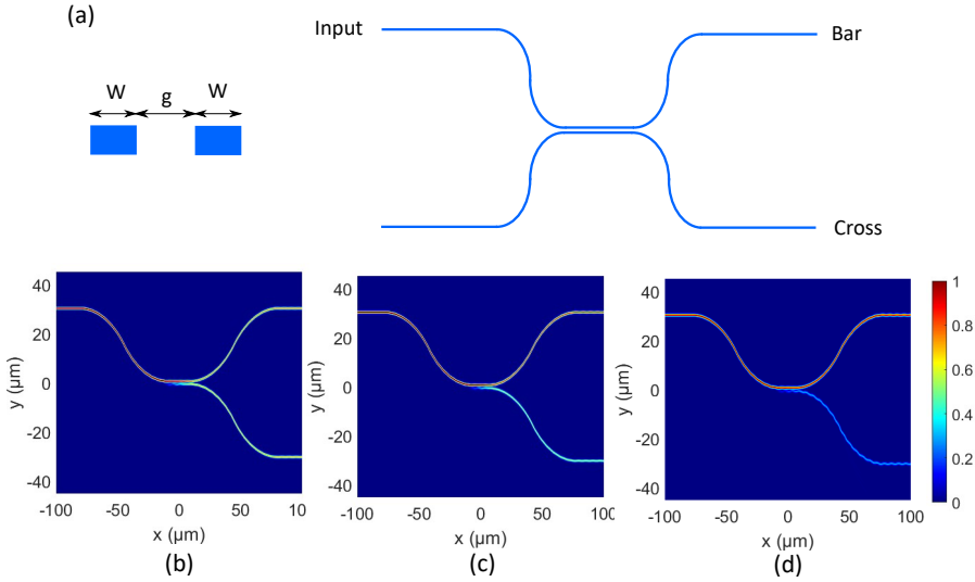
Figure 3.7: (a) Drawing of a straight conventional DC with cross section of the coupling region. VarFDTD simulated power distribution of the DC for K = (b) 0.5 (c) 0.29 (d) 0.08 for the TE mode.
