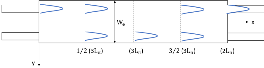
Figure 3.4: Field pattern (represented in blue) in a 2 x 2 MMI when the light comes from the upper input waveguide.
