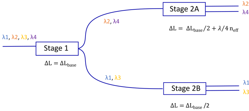
Figure 3.13: Diagram of a cascaded MZI. \lambda is noted as the center wavelength.
