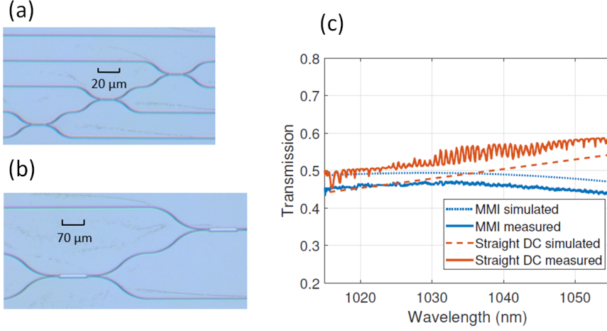
Figure 3.11: Microscope image of (a) cascaded straight DCs and (b) cascaded MMIs). (c) Simulation (dashed curves) and measurements (continuous curves) of straight DCs and MMIs.
