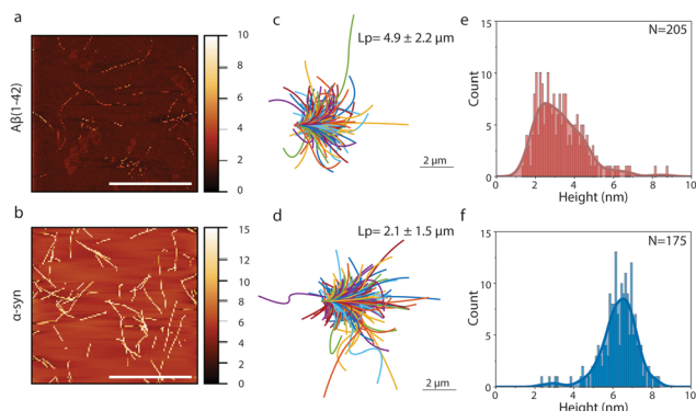
Fig. 3 AFM analysis of amyloid fibril morphology and persistence length. (a and b) Representative AFM image of A \beta (1–42) (a) and \alpha -syn (b) amyloid fibrils. The scale bars are 5 \mu m. (c and d) Contours of A \beta (1–42) ( n = 310 ) (c) and \alpha -syn ( n = 341 ) (d) amyloid fibrils with their initial tangents aligned. The average persistence lengths of depicted fibrils, calculated using the Easyworm software, are indicated in the figure. (e and f) Histograms of fibril height distributions for the A \beta (1–42) (e) and \alpha -syn (f) amyloid fibril samples, the numbers of analyzed individual fibrils are indicated in each graph.
