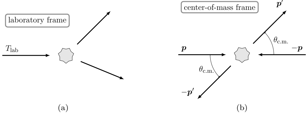
Figure 2.2: Illustration of np scattering seen in the laboratory frame (a) and c.m. frame (b). T_{\text{lab}} denotes the laboratory scattering energy and \mathbf{p} ( \mathbf{p}' ) the ingoing (outgoing) scattering momentum in the c.m. frame.
