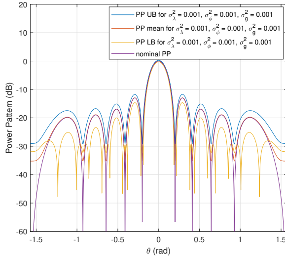
Figure 3.3: Beam pattern deviation bounds based on (3.44), Paper D ©2019 IEEE
