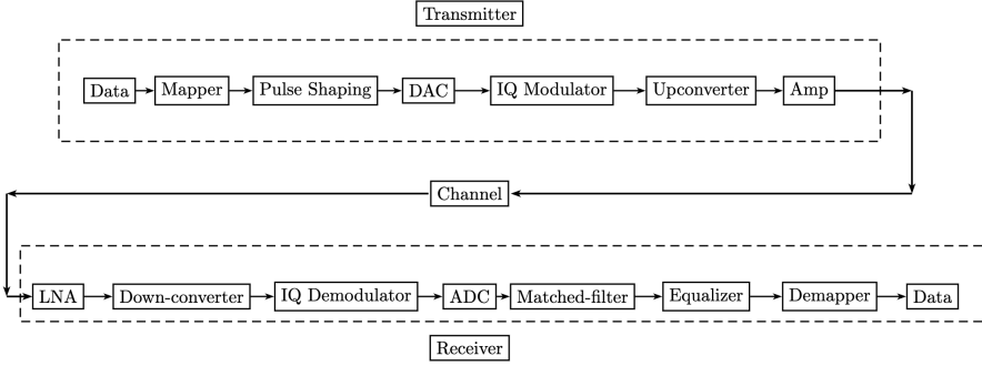
Figure 2.1: Transceiver Block Diagram
