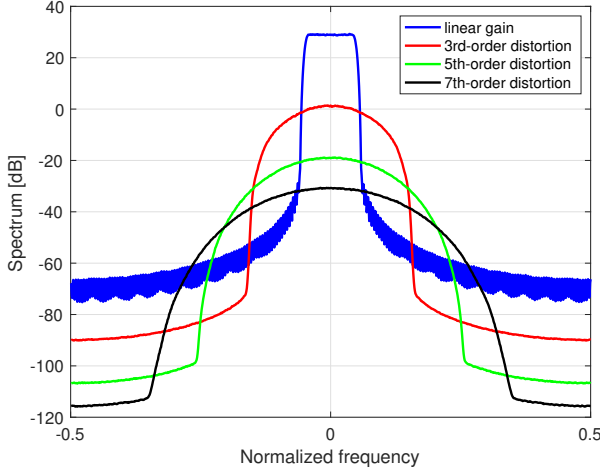
Figure 3.2: PA output linear gain together with higher-order distortions based on measurements for a Gallium Nitride (GaN) power amplifier, the Cree CGH40006-TB model [51] (Fig. 1 in Paper B).
