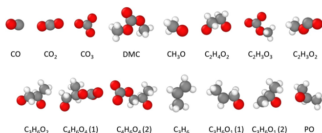
Figure 1. Illustration of the investigated possible electrolyte decomposition products.
