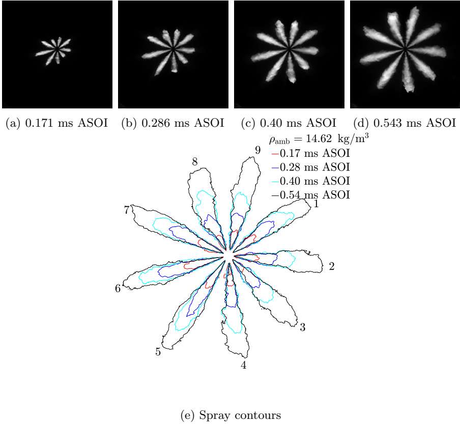
Figure 5.5: Image sequences of multi-plume at \rho_{amb} = 14.62 \text{ kg/m}^3 , P_{inj} = 210 \text{ MPa} , T_{amb} = 298 \text{ K} .
