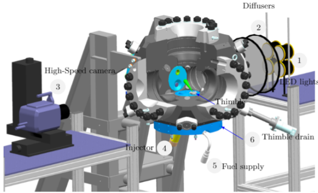
Figure 3.2: Schematic representation of diffuse backlight (DBI) configuration.
