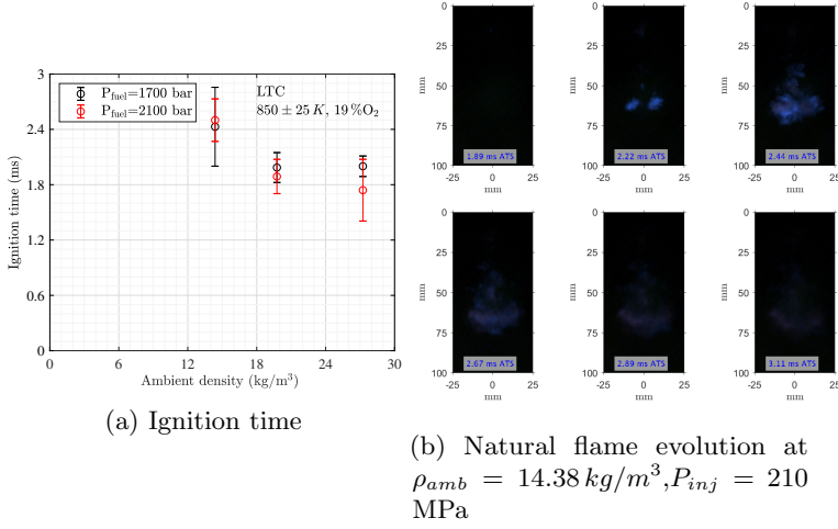
Figure 5.11: Depicting spray flames at 850 K
