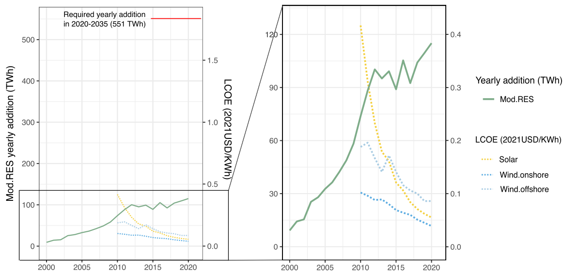
Fig. 4. Costs of solar, onshore, and offshore wind in comparison to yearly addition of modern renewables in the G7 and the EU in 2000–2020 and the required addition in 2020–2035. Note: The costs represent the global weighted average costs of these technologies obtained from IRENA [74].
