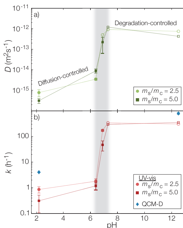
Figure 5.6: a) Fitted diffusion coefficients ( \pm 95\% confidence interval of fit) from microcapsules with an m_s/m_c -ratio of 2.5 and 5.0. b) Fitted rate constants for the polyanhydride degradation based on spectrophotometry and QCM-D. All open markers in both subfigures are modeled threshold values given the temporal resolution of the experiments, and consequently only lower limits.
