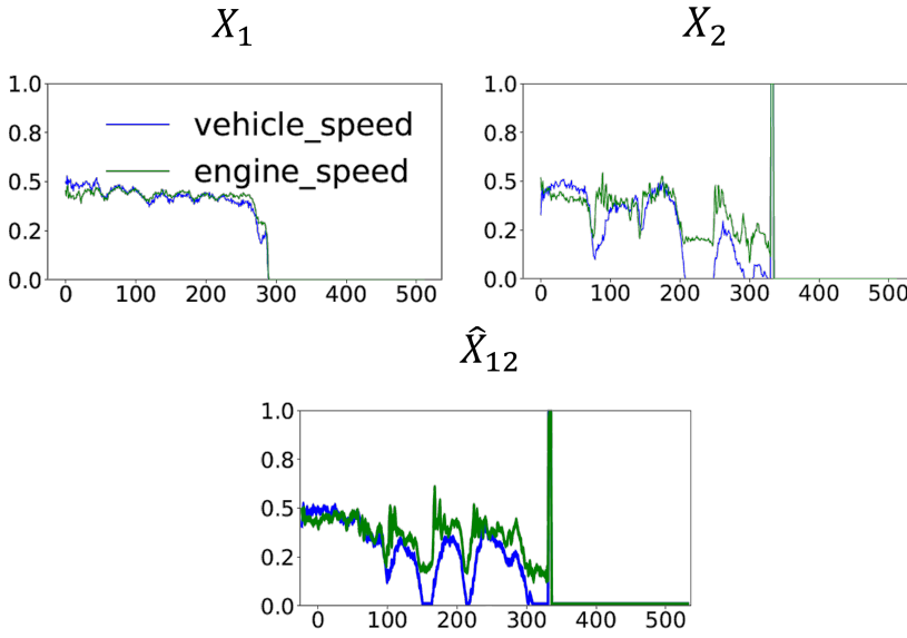
Figure 9.5: Recorded maneuvers of smooth ( X_1 ) and jerky ( X_2 ) stopping, and a generated trace combining both characteristics
