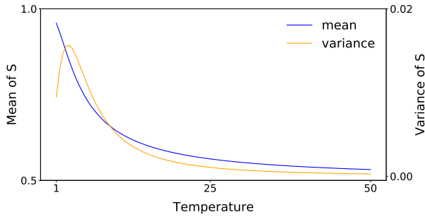
(a) Effect of temperature scaling on the distribution of uncertainty scores F=\text{VGG13}
