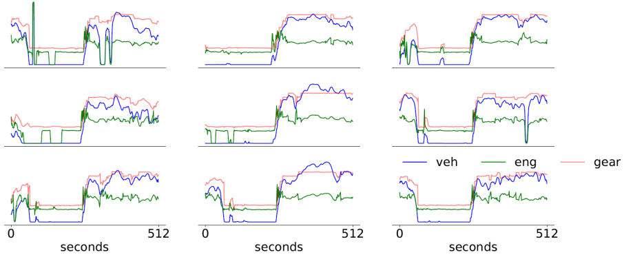
Figure 10.6: Traces generated by simplex sampling in the latent subspace bounded by the three vehicle speed templates
