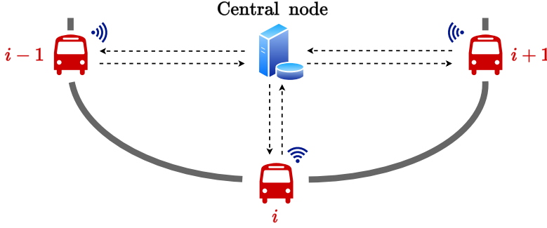
Figure 4.1: Representation of the communication structure between the vehicles and a central computing node in the proposed hierarchical control architecture.
