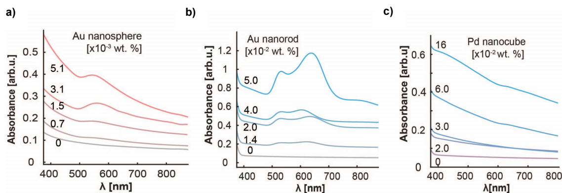
Figure 3.12. UV/Vis spectra 500 \mu\text{m} thick films of a) PLA: Au nanospheres composites, b) PMMA: Au nanorods composites, 2023 and c) PMMA: Pd nanocubes composites. Adapted from Ref. 64 Copyright American Chemical Society 2020 and Ref. 63 Copyright American Chemical Society 2023.
