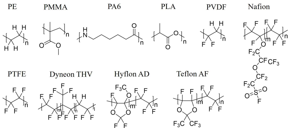
Figure 3.1. Polymer structures.
