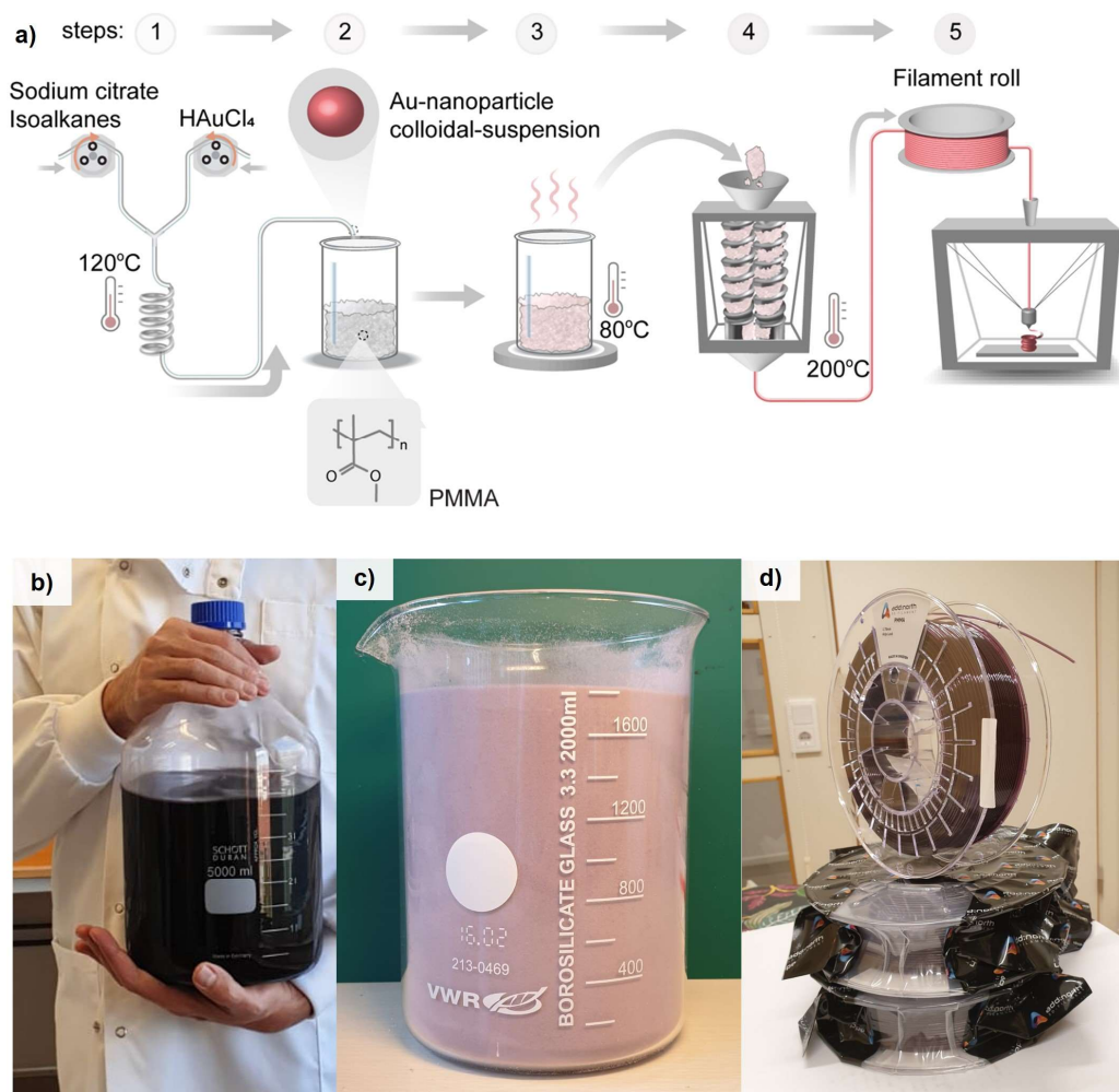
Figure 4.1 Upscaling of plasmonic plastics. a) Processing scheme b) Large scale flow synthesized Au nanospheres in water dispersion. c) PMMA and Au nanosphere powder mixture. d) Three rolls of PMMA: Au nanospheres 3D-printing filament. Adapted from Ref. 63 Copyright American Chemical Society 2023.
