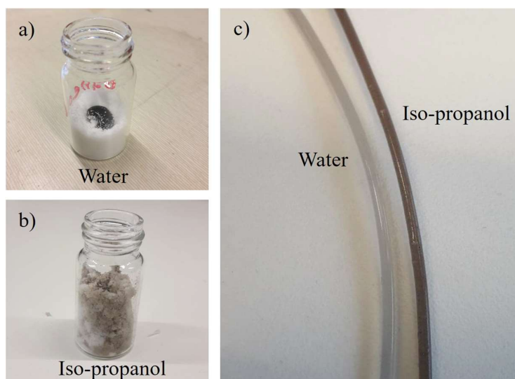
Figure 3.3. Dyneon THV nanocomposite a) Adding Pd nanocubes in water to Dyneon THV powder. b) Adding Pd nanocubes in iso-propanol to Dyneon THV powder. c) Extruded filaments of Dyneon THV: Pd from water dispersion and iso-propanol dispersion.
