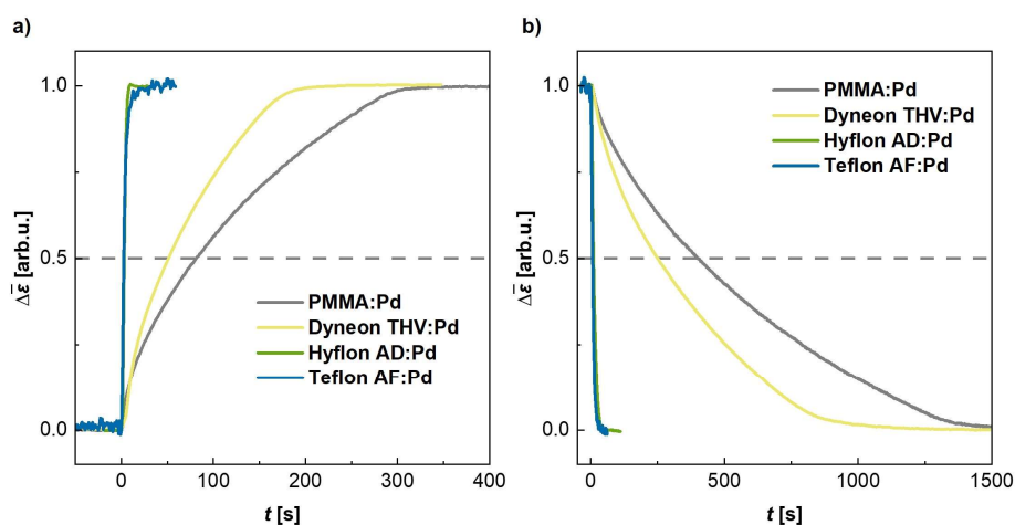
Figure 6.5. Hydrogen sensing of 100 \mu\text{m} thick polymer:Pd plates. a) \Delta\bar{\epsilon} upon a stepwise increase of \text{H}_2 pressure from 0 to 100 mbar. b) \Delta\bar{\epsilon} upon a stepwise decrease of \text{H}_2 pressure from 100 to 0 mbar. Dash grey line denotes 50% of the total signal. Data recorded by Iwan Darmadi.
