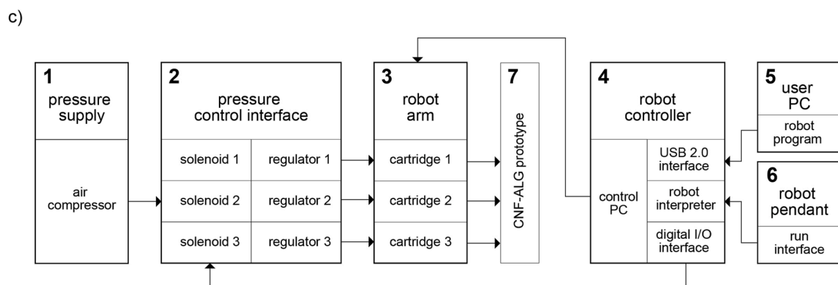
Fig. 1. A) Experiment protocol applied to fabricate the membranes, b) custom-designed robot cell setup for pressure-based extrusion, c) detailed scheme of interconnections between the mechatronic devices, hardware, and user interfaces for pressure-based extrusion within the robot cell.
