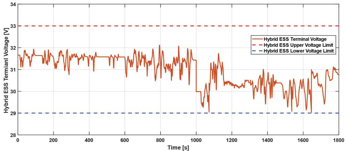
Fig. 11. Hybrid ESS terminal voltage (with lithium-ion cell 5 bypassed). ESS, energy storage system.
