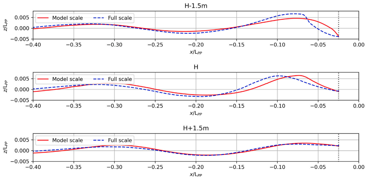
Fig. 25. The longitudinal wave cuts at y/L_{pp} = 0 (at the centre-line) from model and full-scale RANS-VOF computations at H-1.5m, H and H+1.5m loading conditions at 19 kn.
