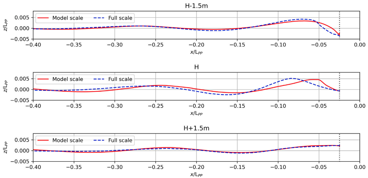
Fig. 23. The longitudinal wave cuts at y/L_{pp} = 0 (at the centre-line) from model and full-scale RANS-VOF computations at H-1.5m, H and H+1.5m loading conditions at 17 kn.
