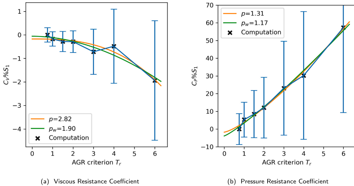
Fig. 2. Computed resistance coefficients relative to the finest grid solution ( S_1 ) with numerical uncertainties as error bars, and observed order of convergences against the AGR criteria.
