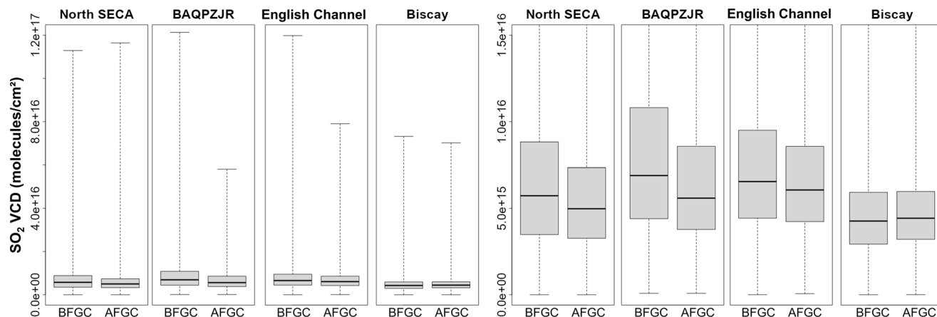
Fig. 6 Impact of global sulfur cap on SO 2 . Box plot of annual SO 2 VCD levels between different areas before (BFGC) and after (AFGC) the global sulfur cap entered into force in 2020, with minimum, 25% percentile, median, 75% percentile and maximum. The left plots include the maximum values, while the right plots give the 25–75% percentile range.
