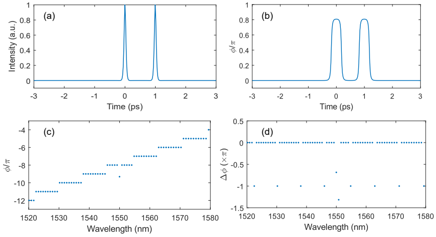
Figure 5.7: Temporal and spectral waveform of the multi-DKS simulated by the Ikeda map in Fig 5.5(b). (a) Temporal pulse profile. (b) Temporal phase profile. (c) Spectral phase of the 100 GHz repetition rate comb modes. (d) Differential phase of the comb modes.
