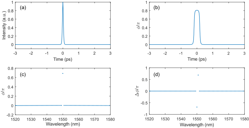
Figure 5.6: Temporal and spectral waveform of the single DKS simulated by the Ikeda map in Fig 5.5(a). (a) Temporal pulse profile. (b) Temporal phase profile. (c) spectral phase of the 100 GHz repetition rate comb modes. (d) Differential phase of the comb modes.
