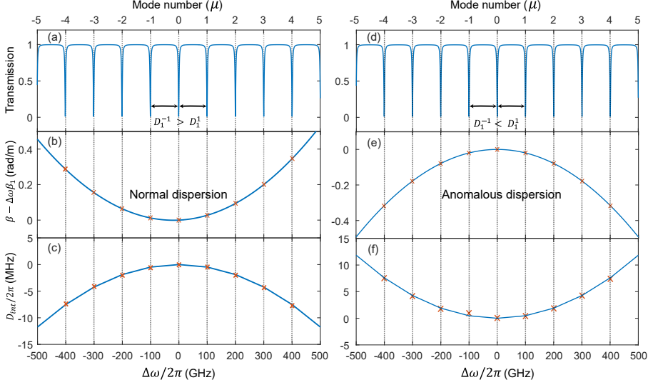
Figure 4.16: Zoom of dispersive ring resonator spectrum simulated from 1535 nm to 1565 nm. a) Transmission profile plot according to equation 4.7 using parameters a = 0.99 , t_1 = 0.96 , t_2 = 0.96 , L = 2\pi \times 238 \mu\text{m} , n_g = 2.1 , \beta_1 = 6 \text{ ps/km} , \beta_2 = 100 \text{ ps}^2/\text{km} with a reference mode \mu_0 at \sim 1550 \text{ nm} and record length of five million. The normal GVD causes a reduction of the FSR towards higher resonance frequencies. b) Taylor expansion of the propagation constant without the effects of \beta_0 and \beta_1 . c) Integrated dispersion plot. The retrieved dispersion from the resonance frequencies is \beta_2 = 99.6 \pm 0.5 \text{ ps}^2/\text{km} . d-f) idem to a-c) but for \beta_2 = -100 \text{ ps}^2/\text{km} . The retrieved dispersion value is \beta_2 = -100.6 \pm 0.5 \text{ ps}^2/\text{km} .
