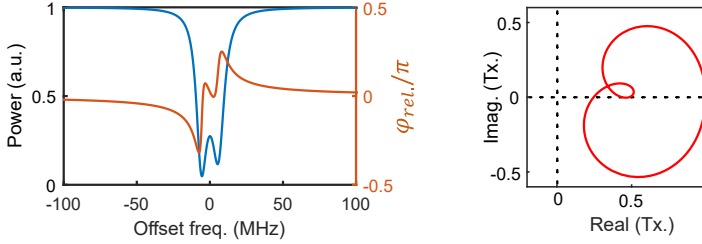
Figure 4.10: Asymmetric resonance split for \kappa_i = 20/2\pi MHz, \kappa_{ex} = 40/2\pi MHz, \kappa_c = (80 + j5)/2\pi MHz. a) Transmission response and phase profile. b) Phasor diagram plot.
