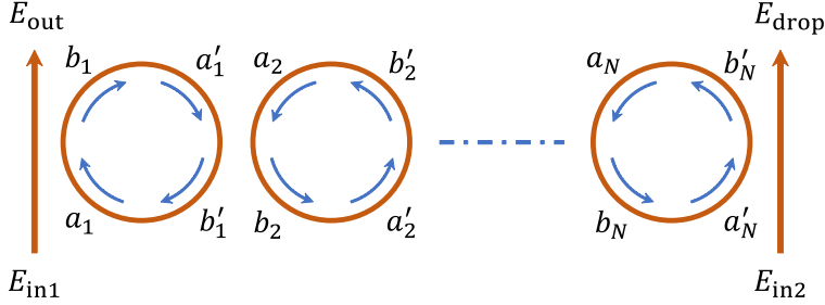
Figure 4.1: Multi-stage traveling wave N resonators with input and output waveguides.
