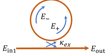
Figure 4.8: A sketch of a single ring resonator with cw and ccw modes.
