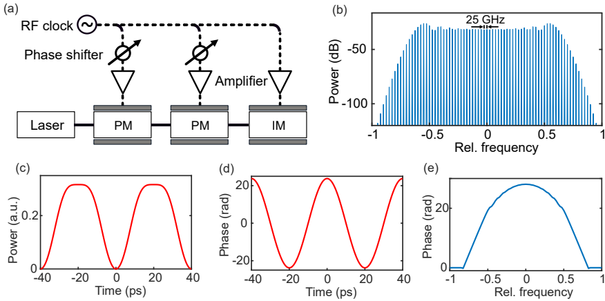
Figure 2.2: (a) EO comb generation setup consisting of two phase modulators and an intensity modulator. The cascaded PM increases the effective modulation depth and the IM flattens the output spectrum. (b) EO comb spectrum of f_r = 25 GHz. (c) Pulse profile of the EO comb with a period of 1/f_r = 40 ps. (d) Phase in time-domain for modulation depth 11.5. (e) Parabolic phase distribution in the frequency domain.
