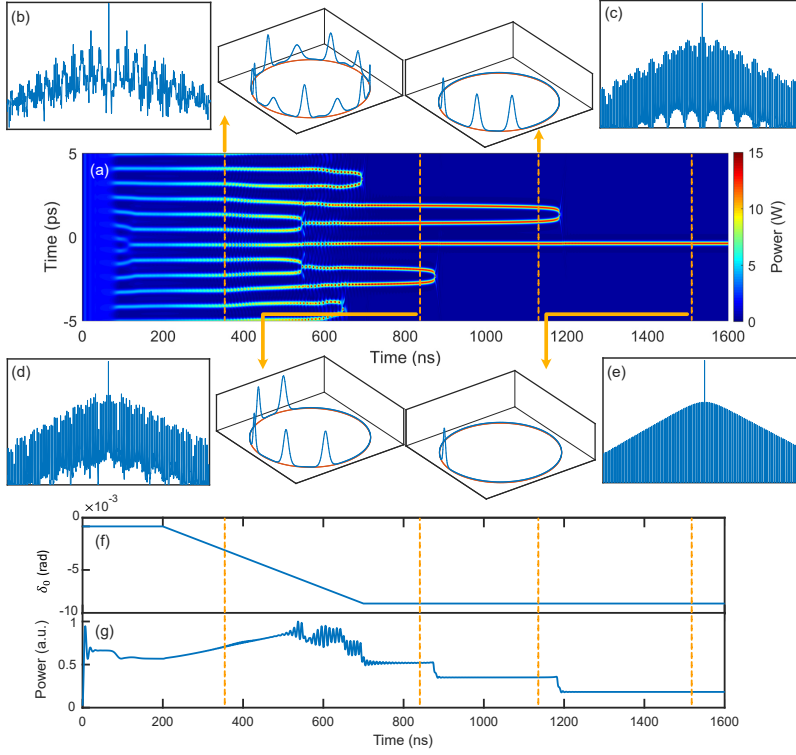
Figure 5.3: Dissipative Kerr soliton dynamics in the microresonator with the parameters: \beta_2 = -150 \text{ ps}^2/\text{km} , \gamma = 1.09 \text{ W}^{-1}\text{m}^{-1} , n_g = 2.1 , FSR=100 GHz, \theta = 0.00034 , P_{in} = 60 \text{ mW} , \alpha = 9 \text{ dB/m} . a) Evolution of the field power in the microresonator. b-e) Spectral response and temporal profile at the different instances of the comb evolution. f) Detuning of the pump from the nearest cold cavity resonance location. g) Intracavity power versus time.
