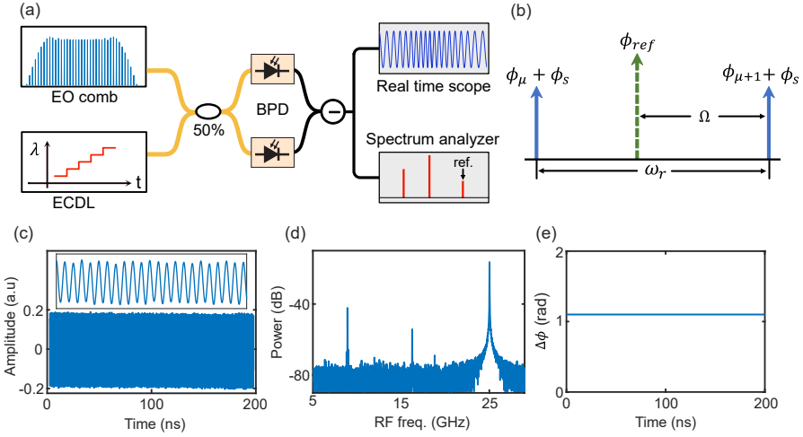
Figure 6.1: Stepped heterodyne optical complex spectrum analyzer. (a) Schematic diagram showing the beating between the EO-comb and reference laser (ECDL). (b) Spectral lines with the corresponding phase. (c) Interference pattern of beat signals and zoom in the inset. (d) RF beat note spectrum. (e) Differential phase of the one pair of the EO-comb lines. ECDL: External cavity diode laser, BPF: Balanced photodiode.
