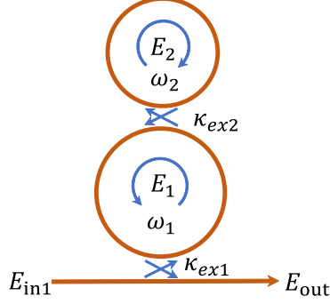
Figure 4.11: . A sketch of linearly coupled ring resonators.
