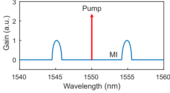
Figure 5.2: MI gain spectrum (blue) with the CW pump (red) plot using parameters: \gamma = 2 \text{ W}^{-1}\text{m}^{-1} , P = 100 \text{ mW} , \beta_2 = -100 \text{ ps}^2/\text{km} , \delta_0 = 0.005 \text{ rad} , L = 150 \text{ mm} , n_g = 2 .
