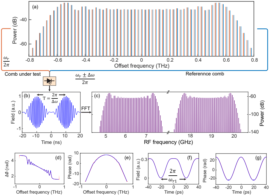
Figure 6.3: Simulation of multiheterodyne spectroscopy. (a) EO combs with a 50 MHz difference in the repetition rate (red: 25 GHz CUT and blue: 25.05 GHz reference comb). (b) Interferogram of period 20 ns. (c) Radio frequency spectrum of two detuned combs. Features of the CUT (red: actual and blue: recovered): (d) Differential phase spectrum, (e) spectral phase profile, (f) pulse profile, and (g) temporal phase profile.
