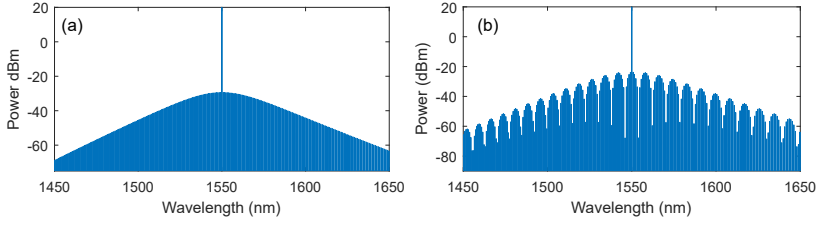
Figure 5.5: Simulated 100 GHz single (a) and multisoliton (b) combs. The comb parameters are as follows: \alpha = 3 dB/m, \beta_2 = -65 ps 2 /km, FSR = 100 GHz, n_g = 2.1 , \gamma = 1 W -1 m -1 , \delta_0 = 0.028 rad, P_{in} = 20 dBm, \theta = 0.0014 .
