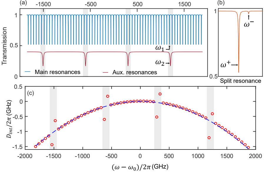
Figure 4.17: Illustration of the mode splitting and implication on the model dispersion of the coupled cavity system using parameters a = 0.94 , t_1 = 0.99 , t_2 = 0.996 , n_g = 2.1 , R1 (main cavity) = 400 \mu\text{m} , R2 (auxiliary cavity) = 25.1 \mu\text{m} , \omega_0 at 1550 \text{ nm} , \beta_1 = 6 \text{ ps/km} at 1565 \text{ nm} , and \beta_2 = 1000 \text{ ps}^2/\text{km} at 1565 \text{ nm} . a) Transmission spectrum of the detached main and auxiliary cavity (offset by 0.5) according to equation 4.7. b) An avoided mode-crossing of uncoupled resonances at \omega_1 and \omega_2 according to equation 4.25. c) Integrated dispersion plot of the uncoupled main cavity (blue line) and coupled cavity (red circles).
