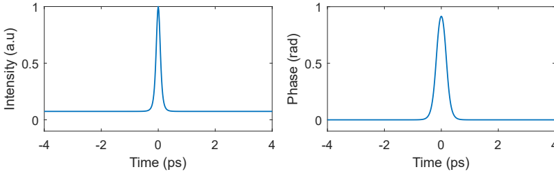
Figure 5.4: Temporal soliton pulse (a) and phase profile (b). The parameters are as follows: \beta_2 = -65 \text{ ps}^2/\text{km} , \delta_0 = 0.028 \text{ rad} , \gamma = 1 \text{ W}^{-1}\text{m}^{-1} , n_g = 2.1 , FSR=100 GHz, \theta = 0.0014 , \alpha = 3 \text{ dB/m} , P_{\text{in}} = 20 \text{ dBm} .
