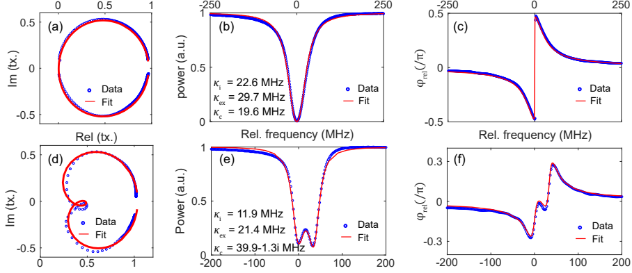
Figure 4.15: IQ plane fitting of the resonances (blue measured and red fitting). Critical coupled resonance (a) IQ plane plot, (b) resonance transmission profile, (c) Phase profile. d-f) idem to a-c) but for asymmetric split resonance.
