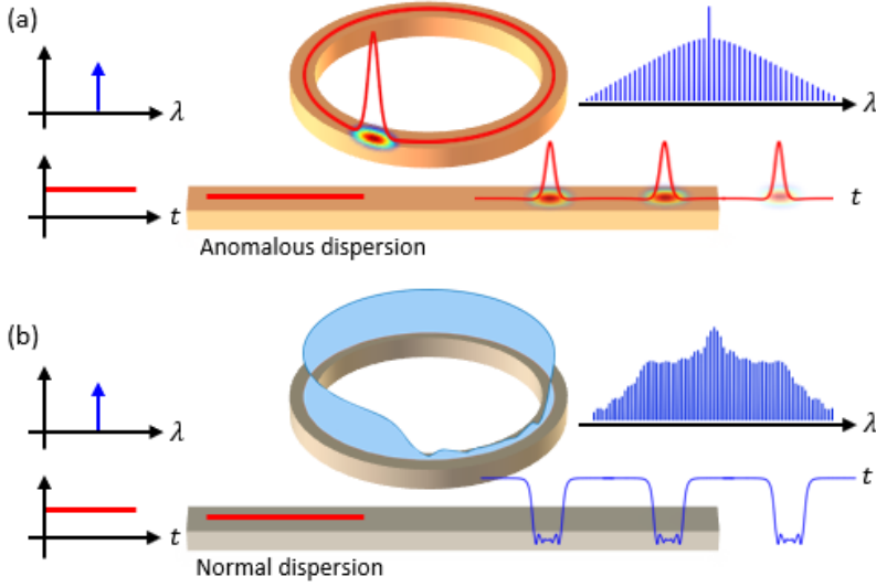
Figure 2.3: Microresonator combs driven by a CW laser. The spectral and temporal profile of (a) dissipative Kerr soliton and (b) dark pulse comb.
