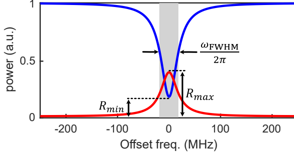
Figure 4.7: Lorentzian shaped spectral response (blue for output and red for drop ports) of the add-drop ring resonator for \kappa_i = 80/2\pi MHz, \kappa_{ex1} = 70/2\pi MHz, and \kappa_{ex2} = 60/2\pi MHz.
