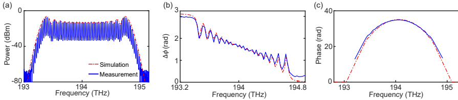
Figure 6.2: Stepped heterodyne complex spectrum analysis of the EO comb (red: simulation and blue: measurement). (a) EO comb spectrum. The modulation depth was set to 14.25 in the simulation. (b) Differential phase profile. (c) Reconstruction of the spectral phase response.
