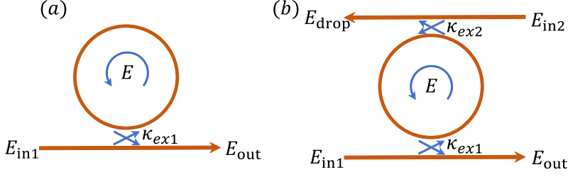
Figure 4.6: A sketch of a single ring resonator. a) All-pass ring resonator. b) Add-drop ring resonator. The field inside the resonator has a unit of the square root of joule and the square root of watt or joule per second for fields outside.
