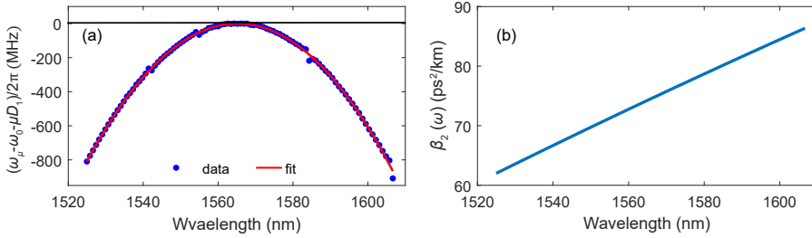
Figure 4.18: (a) Deviation of the resonance frequencies ( D_{int} ) from an equidistant frequency grid \omega_0 + D_1\mu (gray line), where the reference mode is at 1565 nm. (b) Second-order dispersion plot of the microresonator.
