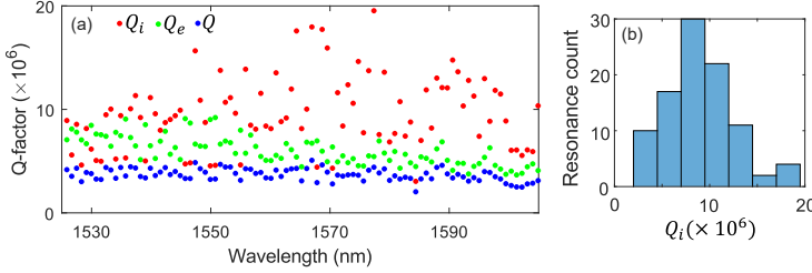
Figure 4.5: a) Quality factor plot of the high- Q resonator of average intrinsic Q_i = 9 million. b) Histogram plot of the intrinsic Q .
