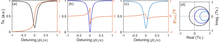
Figure 4.4: Different resonance conditions for the all-pass resonator. Normalized power transmission and phase profile: a) Overcoupling ( a = 0.9, t_1 = 0.8 ), b) Undercoupling ( a = 0.8, t_1 = 0.9 ), Critical coupling ( a = t_1 = 0.9 ). d) Resonances in the complex plane.
