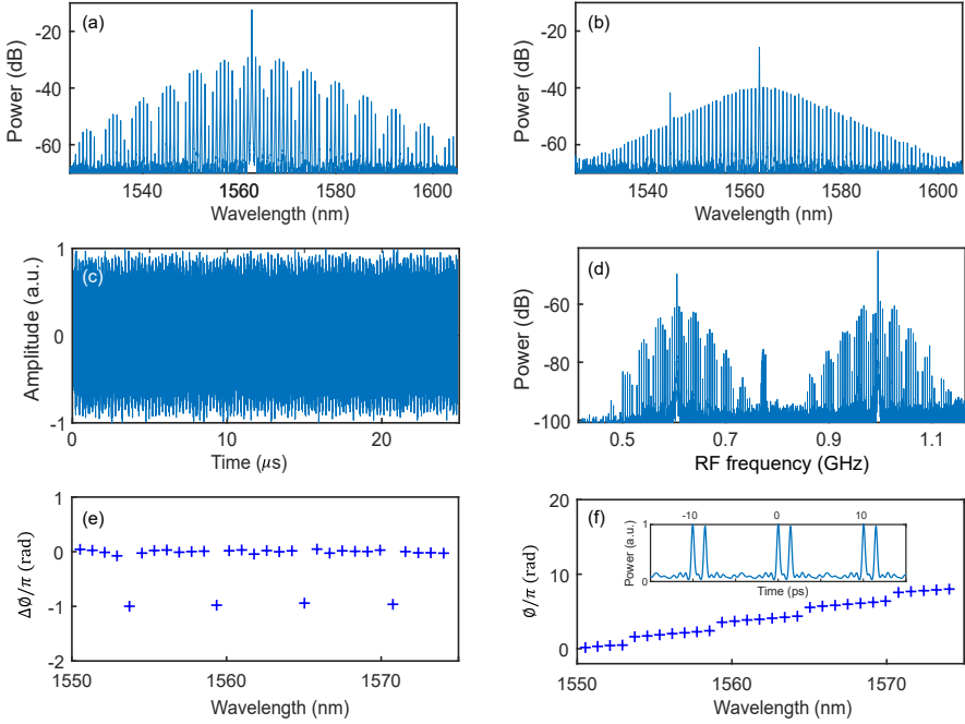
Figure 6.4: Multi-heterodyne spectroscopy of the coupled cavity soliton comb. (a) Multisoliton CUT with pump at 1562.65 nm. (b) Single soliton reference comb with pump at 1563.2 nm. (c) Interferogram recorded for 25 \mu\text{s} of period 0.2 \mu\text{s} . (d) RF comb spectrum after Fourier transform of the interferogram. (e) Differential phase showing \pi periodic phase discontinuities. (f) Phase of the comb lines (Inset: reconstructed pulse profile.)
