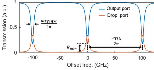
Figure 4.3: Normalized spectra at the output port and drop port with the following parameters: a = 0.93 , t_1 = 0.95 , t_2 = 0.95 , n_g = 2.1 , L = 2\pi \times 225 \mu\text{m} . The abscissa is offset frequency with regard to the center resonance 1550 nm.
