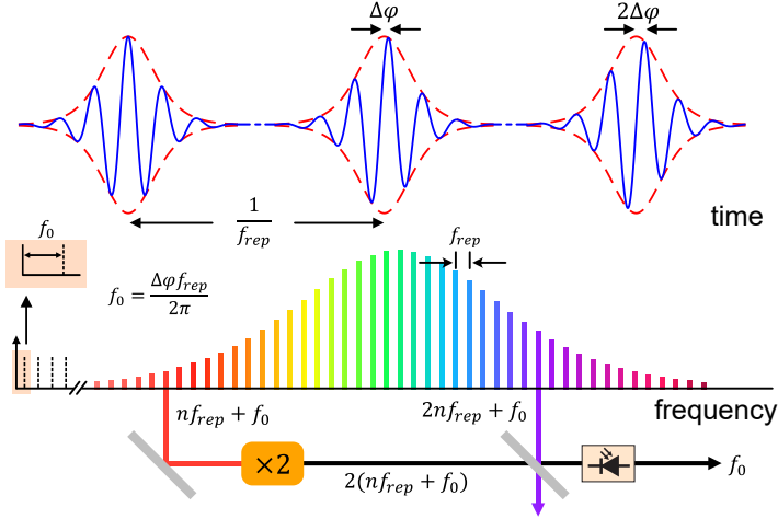
Figure 2.1: Temporal and spectral profile of a femtosecond optical frequency comb. The bottom is the f-2f interferometry for the self-referencing of the comb.
