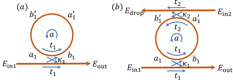
Figure 4.2: A sketch of a single ring resonator. Note 'a' is related to the attenuation factor and with subscript 'a n ' to the field in the ring. a) All-pass ring resonator. b) Add-drop ring resonator.
