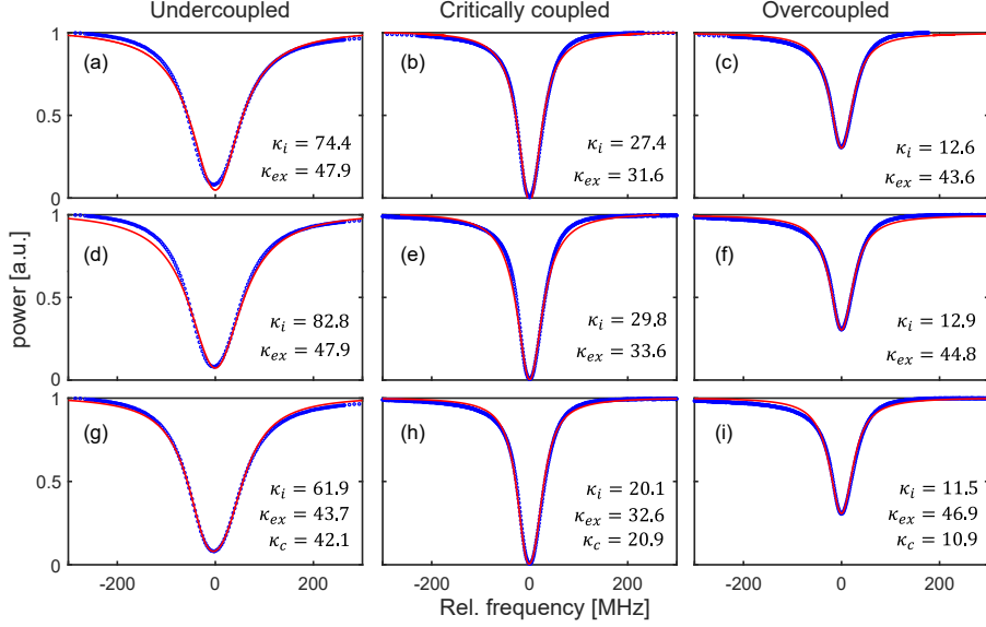
Figure 4.14: Normalized transmission spectra (blue) and parametric fitting profiles (red) of undercoupled, critically coupled, and overcoupled resonances in columns. Each column has identical raw data at different locations of the resonance spectrum. The coupling rates have a unit of MHz. (a-c) Lorentzian lineshape fitting model. (d-f) Parametric coupled mode resonance fitting neglecting ccw mode coupling. (g-i) Parametric coupled mode resonance fitting considering ccw mode coupling.
