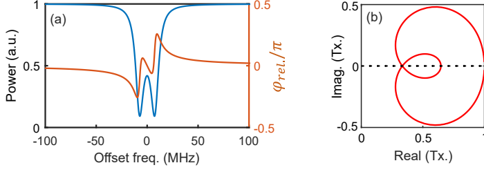
Figure 4.9: Symmetric resonance split for \kappa_i = 20/2\pi MHz, \kappa_{ex} = 40/2\pi MHz, \kappa_c = 100/2\pi MHz. a) Transmission response and phase profile. b) Phasor diagram plot.
