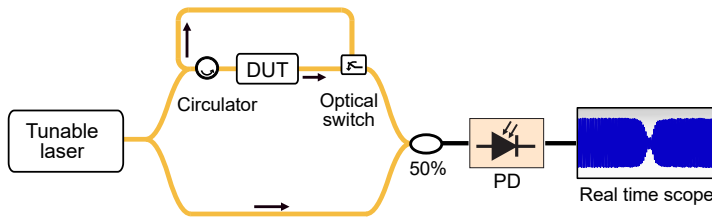
Figure 3.1: Typical Swept wavelength interferometry setup including a DUT. The optical switch configures the transmission or reflection arrangement of the SWI.
