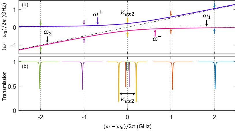
Figure 4.12: Interaction between resonances of the linearly-coupled cavities. a) Illustration of the avoided mode-crossings. The uncoupled modes \omega_1 and \omega_2 , coupling rate \kappa_{ex2} , and supermodes \omega^+ and \omega^- are labeled. The resonance of the first cavity \omega_1 is considered as a reference mode. b) Supermodes distribution of the resonances at the location marked in a) with arrows of identical colors. The spacing between the coupled resonances complies with the supermodes gap in a). At the mode crossing point, the distance between the supermodes (\omega^+ - \omega^-)/2\pi = \kappa_{ex2} .
