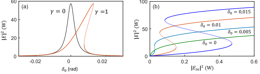
Figure 5.1: Bistability curves showing the intracavity power against a) detuning for |E_{in}|^2 = 75 mW and b) pump power for \gamma = 1\text{W}^{-1}\text{m}^{-1} using parameters: \alpha = 3 dB/m, \theta = 0.005 , L = 226 \mu\text{m} .
