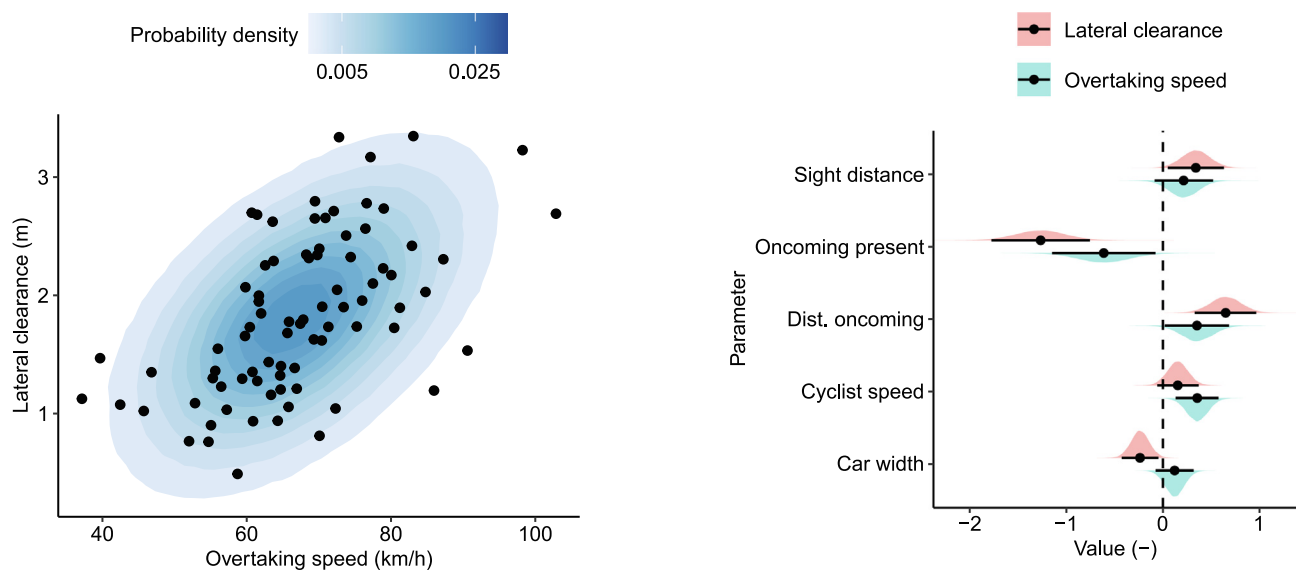
Fig. 7. Model coefficients with full posterior distribution and median (black dot) with 95% highest density interval (HDI, black horizontal bar) marked, for the dependent variables lateral clearance and overtaking speed. All continuous coefficients are on a standardized scale.
