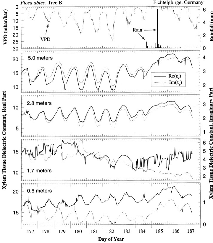
Figure 2.2: Plots of Vapour-Pressure Deficit (VPD) (an indicator of favourable transpiration conditions), rainfall, relative dielectric constant real part \epsilon' and imaginary part \epsilon'' at P-band and at four heights in the stem of a Norway spruce ( Picea abies [L.] Karst) tree. The VPD reference is set to the top of the graph, normalized to the standard atmospheric conditions at sea level (1013 mbar). ©2002 IEEE. Reprinted, with permission, from [31].
