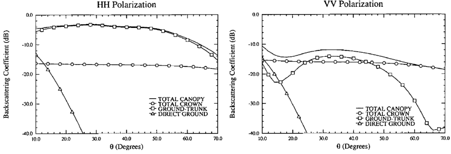
Figure 2.4: Example of simulated L-band backscatter components of a forest using the MIMICS model in [37].
