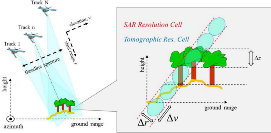
Figure 2.1: Illustration of a TomoSAR acquisition geometry and the resulting resolution cells compared to that of SAR (a single flight track). \Delta r is the range resolution, \Delta \nu the elevation resolution and \Delta z the corresponding vertical resolution. ©2011 IEEE. Reprinted, with permission, from [26].
