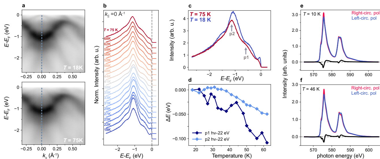
Fig. 4 Temperature dependent ARPES and XMCD measurements. a Example ARPES spectra at temperatures below ( T = 18 K, top) and above ( T = 75 K, bottom) T_N , measured using a photon energy of 22 eV and LH polarised light. b Temperature evolution of the energy distribution curve (EDC) extracted at the \Gamma -point (dashed lines in a ). c Comparison of the high and low-temperature EDCs showing clear additional broadening at high temperatures, as well as peak shifts to higher binding energy. d Extracted energy shift of peaks p1 and p2 from fits to such EDCs as a function of temperature. e, f X-ray absorption spectra across the Cr L_{2,3} edge with left- (blue curve) and right- (red curve) circularly polarised light, measured in an applied magnetic field of 1.4 T, together with the associated XMCD signal (black curve). These spectra were also measured e below (10 K) and f above (46 K) the magnetic transition.
