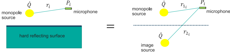
Figure 2.3: Image source principle for monopole radiation over hard reflecting surface.
