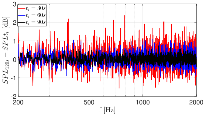
Figure 2.9: Relative difference of SPL between long and shorter sampling times.
