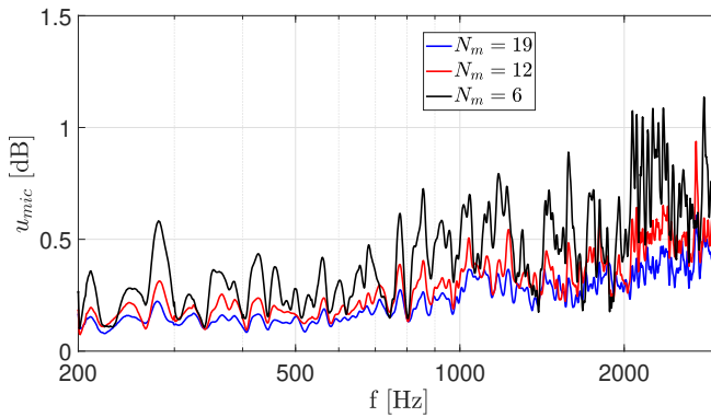
Figure 2.8: Uncertainty due to finite number of microphone positions.
