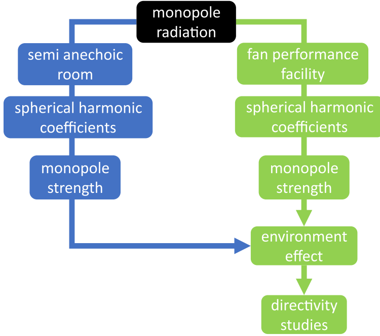
Figure 2.6: Outline of approach based in spherical harmonic decomposition.
