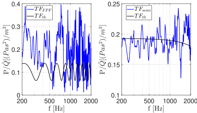
Figure 2.4: Comparison of theoretical TF_{th} and measured TF_{me} for monopole radiation: FPF (left) and semi anechoic room (right).
