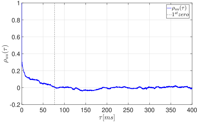
Figure 2.10: Representative estimate of \rho_{uu}(\tau) upstream of low-speed axial fan.
