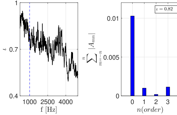
Figure 2.7: Relative monopole strength \iota over frequency (left) and spherical harmonic coefficients magnitude at 1000 Hz (right).
