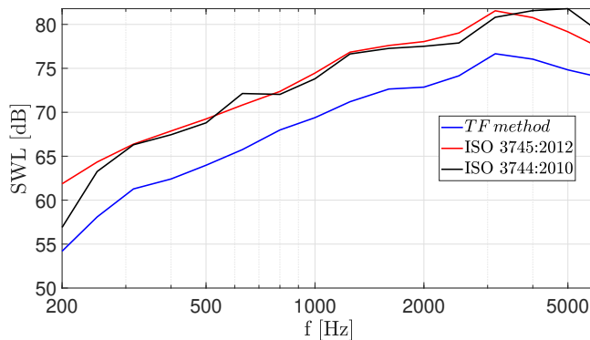
Figure 2.5: Comparison of SWL from monopole source: TF method, ISO 3744:2010 [49] with K_2 and ISO 3745:2012 [40] for semi anechoic.
