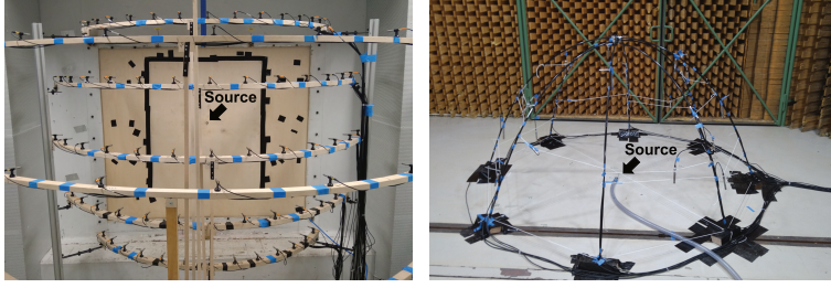
Figure 2.2: Measurement setup of monopole source at FPF (left) and semi anechoic room (right).
