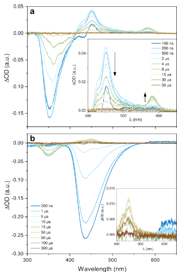
Figure 5. Transient absorption spectra of (a) 8 mM N-1TMS and 25 \mu\text{M} 4CzBN in deaerated toluene and (b) 0.1 mM N-1TMS and 25 \mu\text{M} 4CzBN; t_{\text{ex}} = 410 nm, 1.4 mJ/pulse. Insets show the absorption features of relevance.
