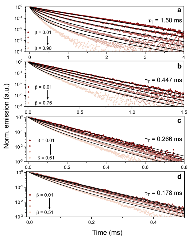
Figure 3. Time-resolved upconverted emission of 25 \mu\text{M} 4CzBN and N-2TMS for different [^1A]_0 . (a) [^1A]_0 = 100 \mu\text{M} , (b) 1 mM, (c) 2 mM, and (d) 3 mM. Emission measured at 375 nm upon 405 nm pulsed excitation at different intensities ranging from 56 \text{mW cm}^{-2} to 17.5 \text{W cm}^{-2} . Black lines are the best global fits of eq 1 using a shared \tau_T . Note that the time scales are different for each panel.
