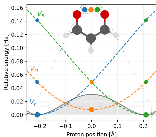
Figure 1. A schematic image of the potentials ( V_R , V_M , V_L ) associated with the three reference Hamiltonians \hat{H}_R , \hat{H}_M , \hat{H}_L defined in the main text and used throughout this work. The inset malonaldehyde shows the transition state structure with “Left”, “Middle”, and “Right” settings for a proton. Apart from the discrete points shown, the potential energy curves are not exact and merely serve to provide the reader with a general guide. The curves were generated by fitting a third-order polynomial to the three points corresponding to each Hamiltonian. The gray shaded area is the scaled-up electronic potential energy calculated with MP2 and aims to illustrate the total potential, and in particular the reaction barrier.
