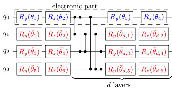
FIG. 5. The “expanded” variant for the initialization of the electronic parameters in hardware-efficient Ansatz . The circuit is designed for the case of four-qubit NEO Hamiltonian, corresponding to H_2 using minimal basis sets, STO-6G for electrons and DZSNB for nuclei. We use an “all-to-all” entangling scheme with CZ gates applied between all qubits. The electronic subsystem is delimited by a dashed box. Parameters in blue are initialized according to the results of the electronic subsystem optimization. All parameters in red: \tilde{\theta}_i ( i = 1, 6 ) and \tilde{\theta}_{d,i} ( i = 1, 6 ) are initialized to 0, with the exception of \tilde{\theta}_{d_{\max},1} , which is set to \pi ( d_{\max} is the maximum number of repetitions). While for this specific case, one entangling layer, d = 1 , would be sufficient, for larger systems, more layers will be required.
