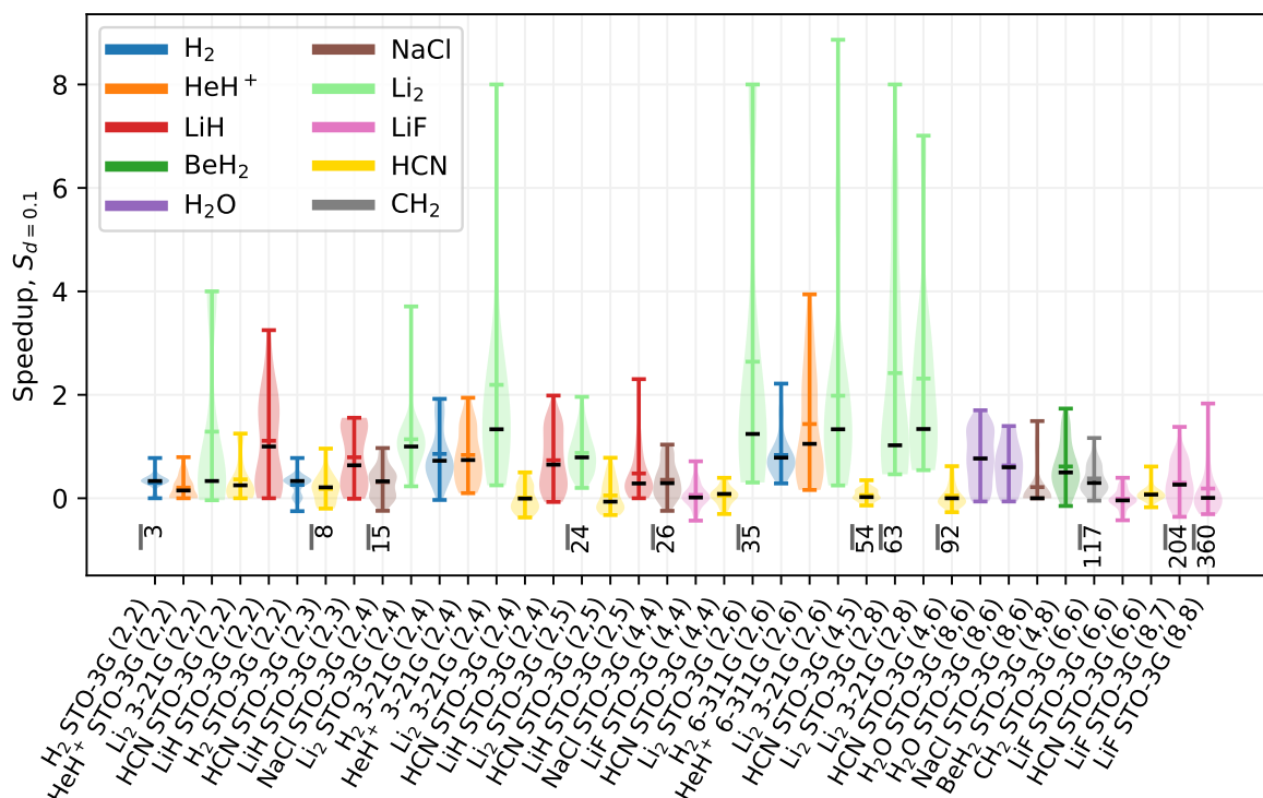
Figure 7.1: Speedup for an assortment of small molecules at a transfer distance d of 0.1 Å. Molecules are sorted according to the number of parameters in the respective VQE ansatz. The width of each violin is in proportion to the number of points along the PES that achieve the given speedup. The figure is reproduced from Paper I.
