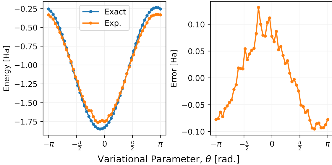
Figure 4.2: Evaluation of the H_2 Hamiltonian on the Chalmers Särimer three-qubit quantum computer, using a one-parameter hardware-efficient ansatz (Figure 4.1). Substantial errors are measured as a result of noise in the quantum calculation. The exact solution, calculated through noise-free simulation, is also shown. Each point in the graph corresponds to 5000 individual readouts of the Hamiltonian terms. Substantial errors are found in the region surrounding the ground state solution.
