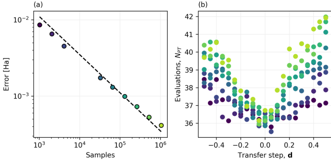
Figure S7: Calculations performed with the COBYLA optimizer using varying number of samples (between 2^{10} and 2^{20} ). The number of samples used for each calculation is indicated by the color of each point. Blue indicates a low number of samples; green indicates a high number of samples. (a) The error decreases (almost) as the standard deviation of a normal distribution \sigma/\sqrt{n} (black line). (b) Average number of function evaluations before PT convergence, N_{PT} for a given transfer step \mathbf{d} . The number of evaluations needed to converge increases with the number of samples.
