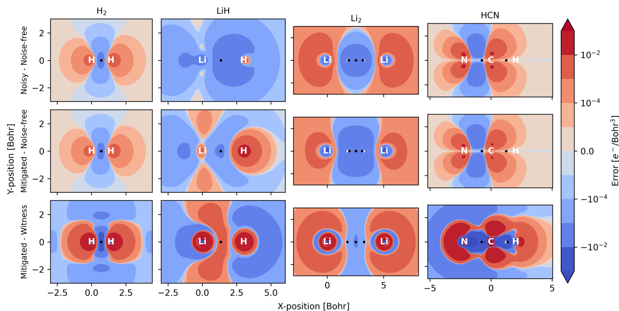
Figure 7.3: Differences in the electron densities between (top) noisy and noise-free (middle) mitigated and noise-free, and (bottom) mitigated and near-exact witness for H_2 , LiH , Li_2 , and HCN . The figure is reproduced from Paper III.
