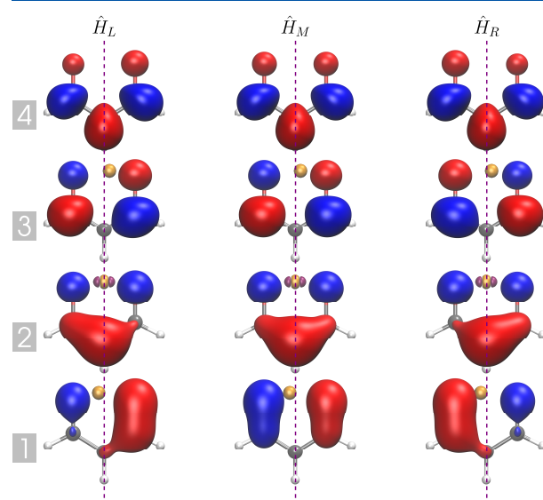
Figure 2. Electronic (red/blue) and nuclear (orange/purple) orbitals (isosurface value is 0.05) included in the active space of NEOCASI calculation for malonaldehyde in the “Left” ( \hat{H}_L ), “Middle” ( \hat{H}_M ), and “Right” ( \hat{H}_R ) setups. The orbitals were prepared with a NEOHF calculation using the DZSNB and 6-31G basis sets for the nuclei and the electrons, respectively.
