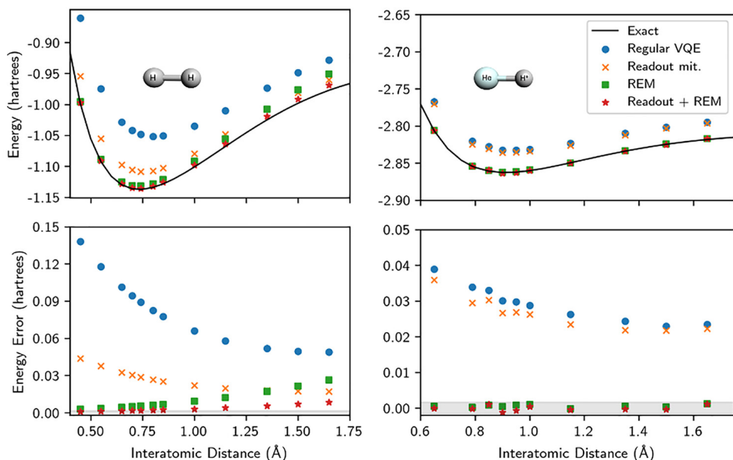
Figure 7.2: Mitigation effects of on the PESs for \text{H}_2 and \text{HeH}^+ . In addition, readout error mitigation is employed. The lower figures show the error, with the shaded region corresponding to 1.6 mHa. The figure is reproduced from Paper II.
