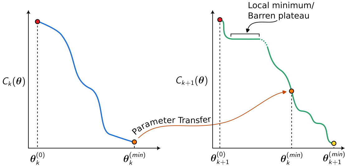
Figure 3.2: Schematic representation of the parameter transfer approach allowing for faster convergence. An initial calculation k is performed and converged for a cost function C_k . The optimized solution, \theta_k^{(min)} , is passed as an initial guess to the next optimization for configuration C_{k+1} . Parameter transfer can help overcome both local minima and barren plateaus.
