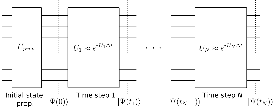
Figure 6.5: Trotterized time evolution circuit. An initial state, |\Psi_0\rangle , is prepared by means of UCC or some other stationary state solver, U_{prep.} . |\Psi_0\rangle is then evolved according to the Trotterized approximation U_k \approx \exp[iH_k \Delta t] .
