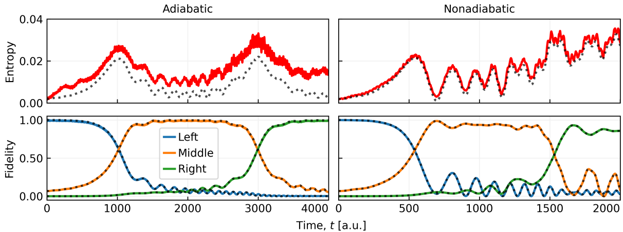
Figure 6.7: Fidelity and proton-electron entanglement during adiabatic (left) and nonadiabatic (right) time evolution. The dashed lines are a near-exact reference calculated using fourth-order Runge–Kutta. The entanglement shows a substantial error in the adiabatic domain, owing to larger time step and insufficient Trotterization used in the time evolution. Figure is reproduced from Paper V.
