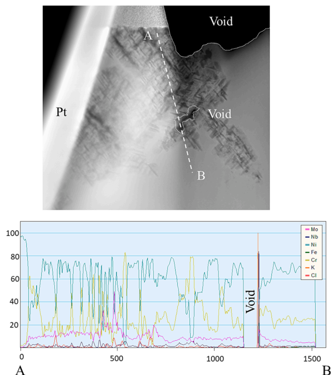
Fig. 9. TEM Line scan analysis of the BIB cross section of Inconel 625 through the internal oxidation zone.
