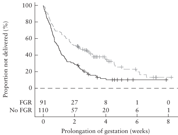
Figure 2 Kaplan–Meier curve showing prolongation of pregnancy in those with (—) and those without (---) coexisting fetal growth restriction (FGR). +, pregnancies that reached 34 weeks' gestation.
