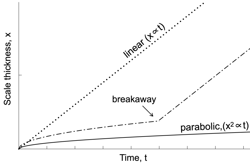
Figure 2.5: Schematic of the ideal rate laws for oxide scale growth at high temperatures: linear growth, parabolic growth, and breakaway oxidation.
