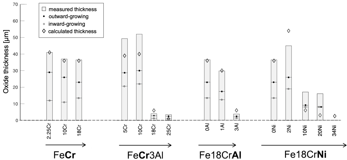
Figure 5.4: Summary of the measured oxide scale thicknesses for all model alloys exposed for 48 hours in 5% O_2 + 95% N_2 + 1 mg/cm 2 K_2CO_3(s) at 600 °C, including estimated thicknesses, calculated from mass gain data, ( \diamond ). Note that the oxide scale formed on the Fe18Cr34Ni alloy was not examined in cross section.
