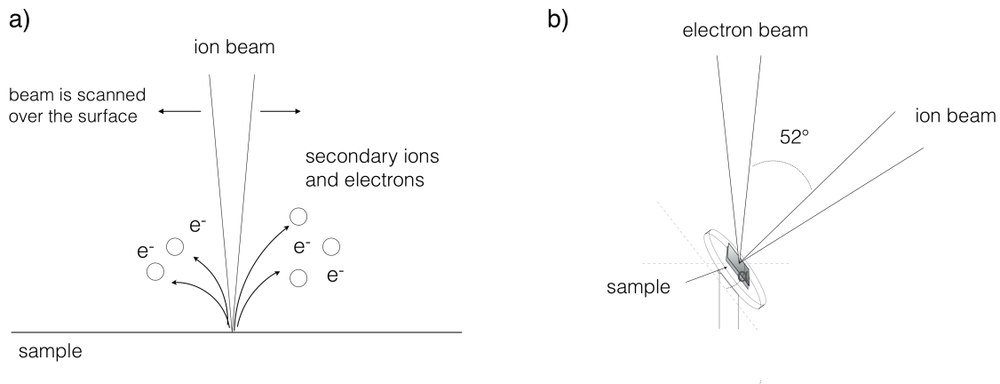
Figure 4.7: Illustration of the image formation in the FIB (a), as reconstructed from [84], and b) a schematic of the SEM/FIB workstation.
