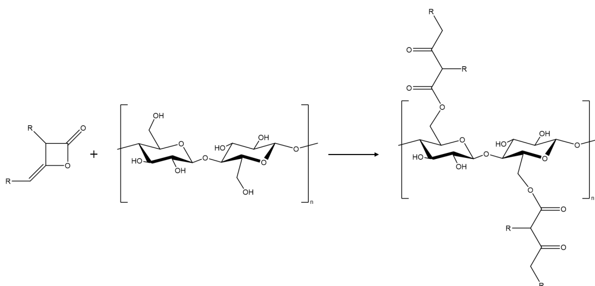
Figure 3. Schematic diagram of the AKD and cellulose reaction.
