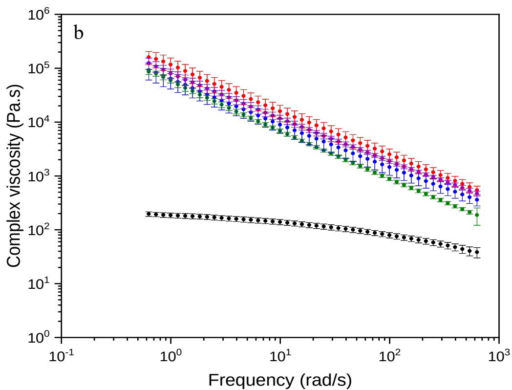
Figure 18. G' (triangles) and G'' (squares), (a) and complex viscosity (circles), (b) as a function of frequency at T=180\text{ }^{\circ}\text{C} and strain= 2.5\text{ rad}^{-1} for PP (black), PP-TMP (blue), PP-TMP AKD Lau (red) and PP-TMP AKD St (green)
