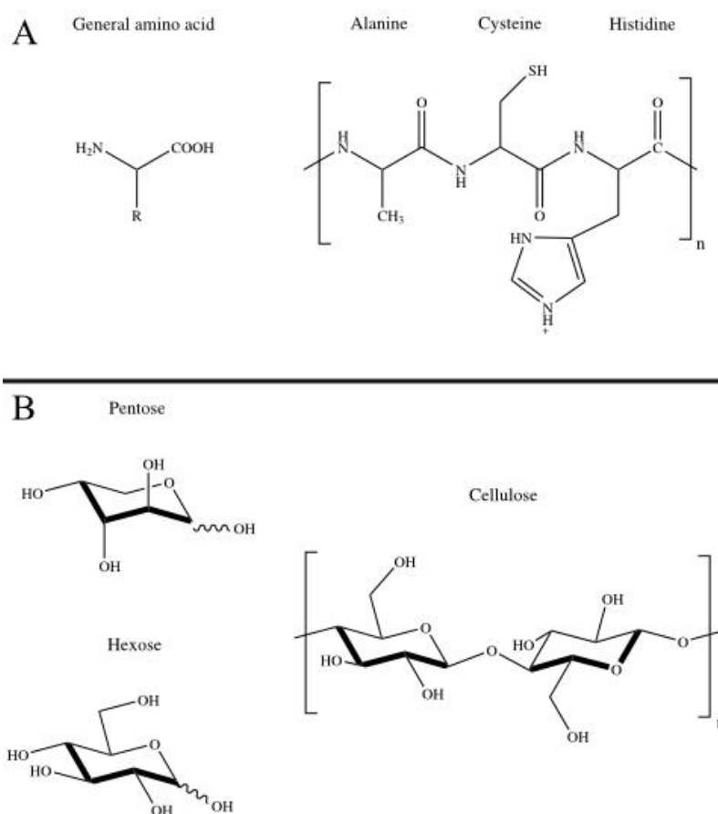
Figure 2.1. Example structure of protein and polysaccharide, and their monomeric units. A. General amino acid structure with amino group ( \text{NH}_2 ), carboxylic group ( \text{COOH} ) and a varying side chain ( -\text{R} ). Example of a polypeptide chain (protein) consisting of alanine, cysteine, and histidine. B. Two common monosaccharide structures, pentose, and hexose. Example of the polysaccharide cellulose built up by the repeating monomeric unit glucose.
