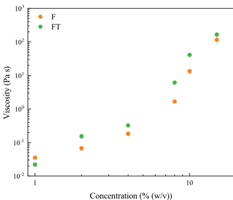
Figure 4.3: Viscosity of non-thermally (F) and thermally (FT) treated pea fibres at six concentrations. Measurements were done in triplicate at 20 °C and a shear rate of 10 \text{ s}^{-1} . The values are an average and error bars not visible are smaller than the symbol.
