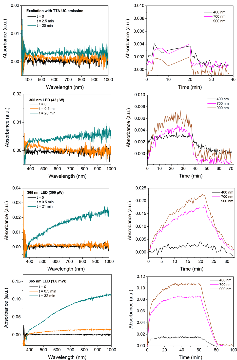
Figure 5.3 Left: UV-Vis absorption spectra of the \text{TiO}_2 film as function of excitation power. The film was excited with TTA-UC emission and with the 365 nm LED with different excitation power (43 \mu\text{W} , 300 \mu\text{W} and 1.6 mW). Right: Absorbance dependence with time for different wavelengths representing the region assigned to \text{TiO}_2(\text{h}^+) (400 nm) and \text{TiO}_2(\text{e}^-) (700 nm and 900 nm).
