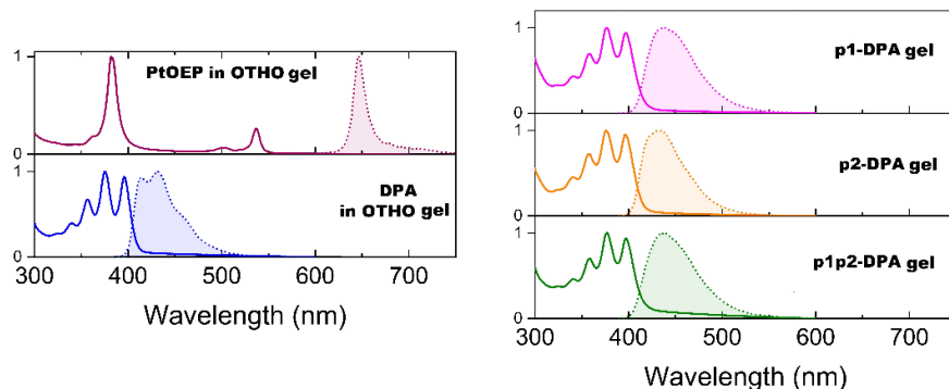
Figure 4.4. Normalized absorption and emission spectra of free PtOEP in OTHO gel (6 \mu M, [OTHO] = 10 mM), free DPA in OTHO gel, p1-DPA , p2-DPA gels ([OTHO-DPA] = 10 mM) and p1p2-DPA gel ([OTHO-DPA] = 5 mM, [OTHO] = 5 mM).
