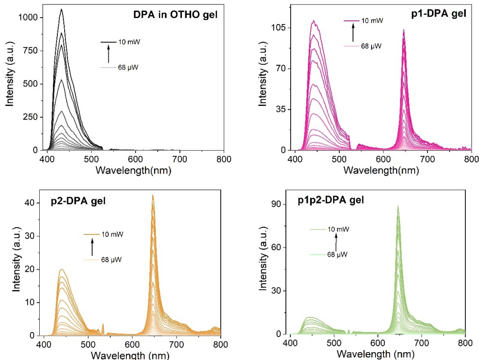
Figure 4.7. Upconverted emission profiles for various DPA samples as indicated in the panels, with excitation power varying from 68 \mu W to 10 mW ( \lambda_{ex} = 532 nm) and remaining PtOEP phosphorescence at 646 nm. ([DPA units] = 10 mM, [OTHO units] = 10 mM, [PtOEP] = 115 \mu M)
