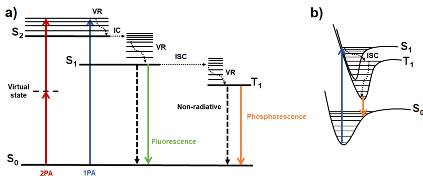
Figure 2.1. (a) Electronic transitions illustrated in a Jablonski diagram showing one (1PA) and two-photon absorption (2PA) processes, and the possible decay paths following absorption. Solid horizontal lines represent energy levels, thinner lines are vibrational levels, and thicker lines are electronic states. Vertical lines represent transitions between states. (b) Illustration of intersystem crossing due to the overlap between the excited singlet and triplet states.
