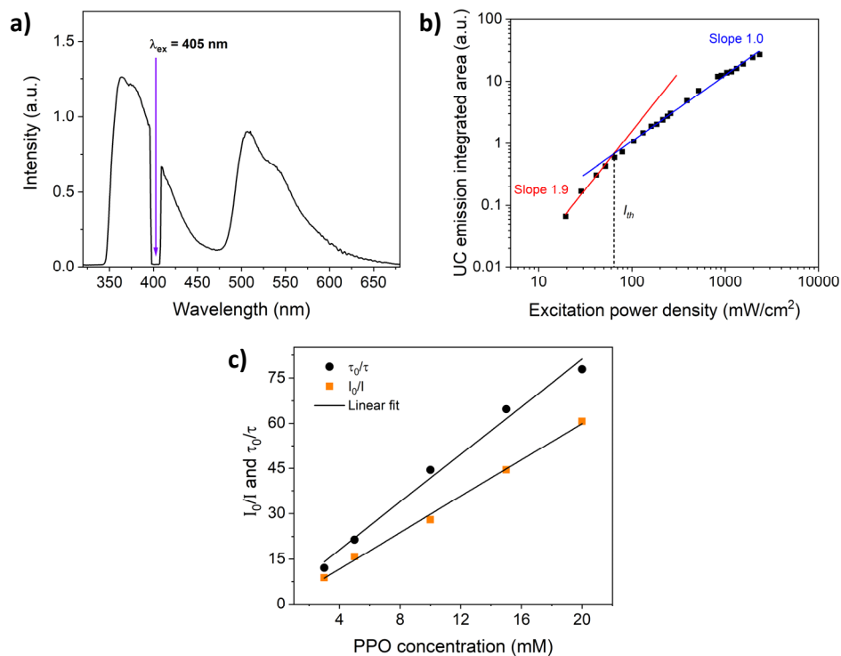
Figure 5.2. (a) Emission spectra with UC fluorescence at 365 nm and unquenched sensitizer phosphorescence at 507 nm. ( \lambda_{ex} = 405 nm, [PPO] = 15 mM, [Ir(p-CF 3 -ppy) 3 ] = 100 \mu\text{M} , in oxygen free acetonitrile). (b) Log-log plot of UC emission integrated area vs. excitation power density, the quadratic and linear regimes of the emission are represented by the linear fittings with slopes 2 and 1, respectively. The cross point is the intensity threshold I_{th} . (c) Stern-Volmer plots for steady state and time resolved data respectively.
