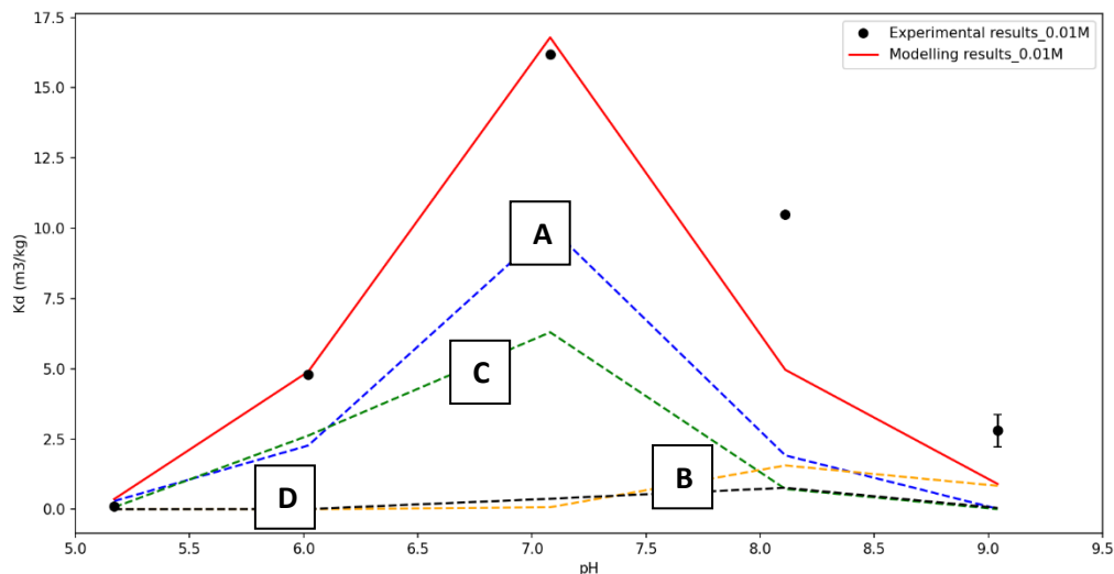
Figure 5-13: An example figure for Eu sorption measurement (symbol) and modelling (continuous line) on biotite mineral in 0.01 M \text{NaClO}_4 solution. The contribution of different Eu(III) species in its sorption is represented by different curves: (A: blue line) \equiv \text{SOEu}^{2+} ; (B: yellow line) \equiv \text{SOEu}(\text{OH})_2 ; (C: green line) \text{EuX}_3 ; (D: black line) \equiv \text{SOEu}(\text{OH})^+
