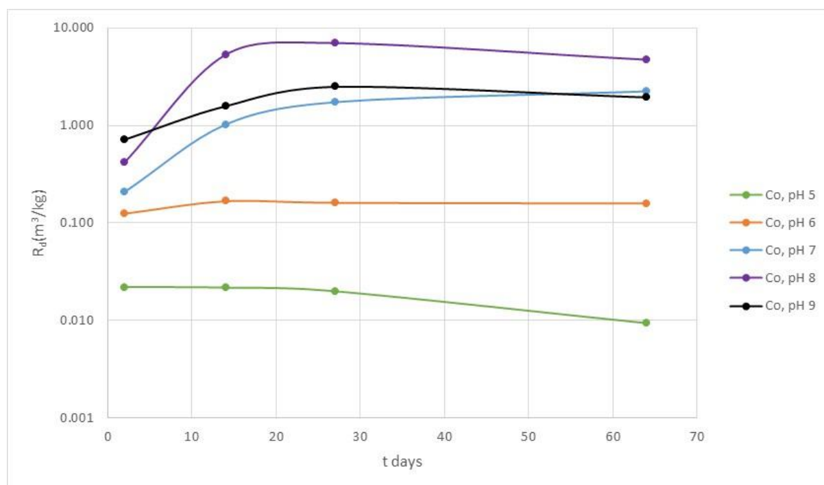
Figure 5-9: Measured R_d values for Co sorption onto biotite in 0.001 M \text{NaClO}_4 versus time.
