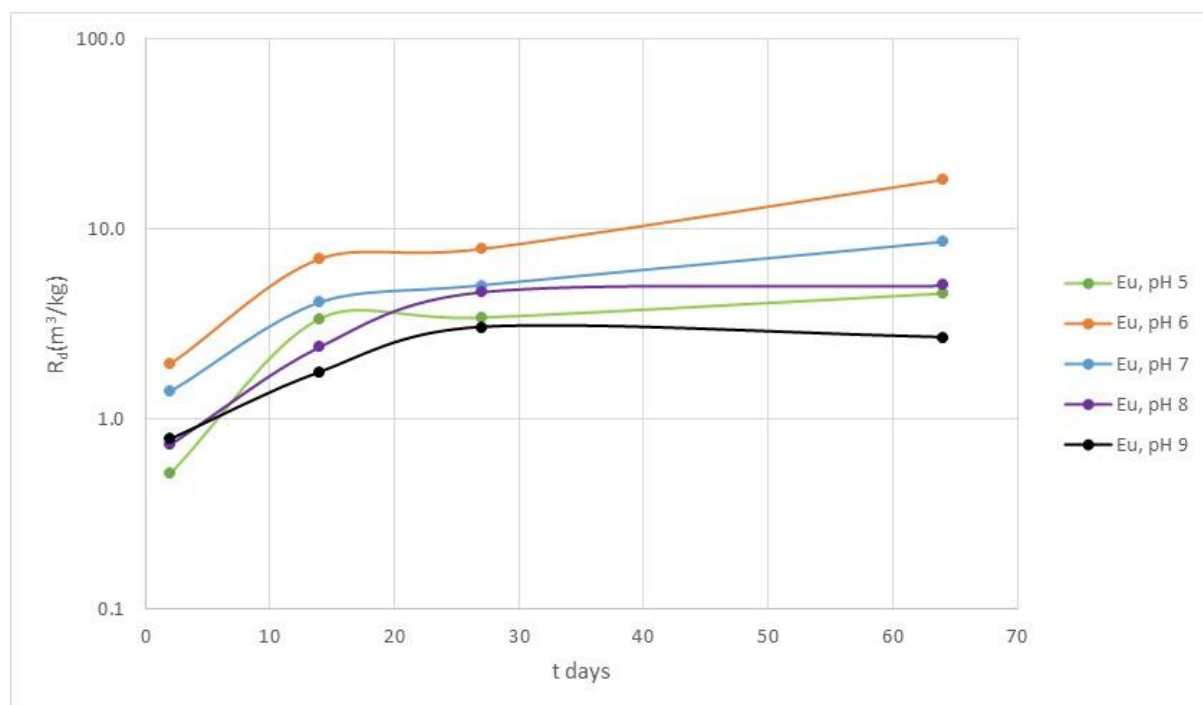
Figure 5-12: Measured R_d values for Eu sorption onto biotite in 0.001M \text{NaClO}_4 versus time.
