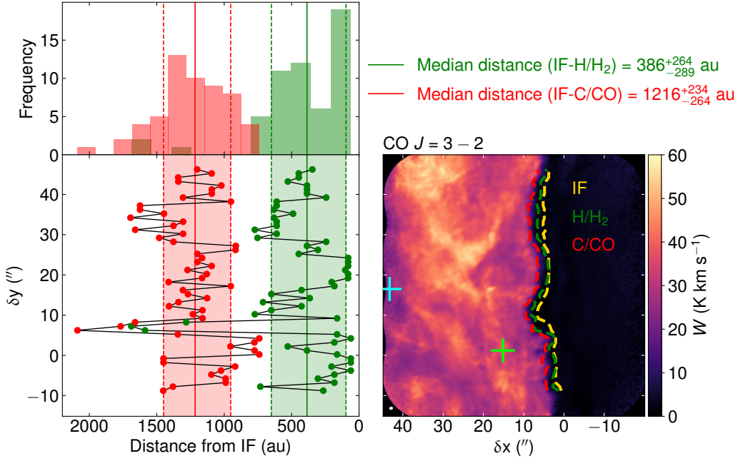
Fig. 5. Location of the ionization, dissociation, and C + /C/CO transition zones. Left: distances of the dissociation front (H 2 /H + , green dots) and C + /C/CO transition zone (C/CO, red dots) with respect to the ionization front (IF) for different \delta y vertical positions. The distributions of the distances are shown in the top panel, where the solid vertical lines represent the median values, and the dashed lines represent the uncertainties based on the 16th and 84th percentiles of each distribution. Right: IF (yellow), H 2 /H + (green), and C/CO (red) transition zones overlaid on top of the CO J = 3 - 2 integrated intensity map. The two crosses mark the PDR and dense core positions. The angular resolution is plotted in the bottom left corner.
