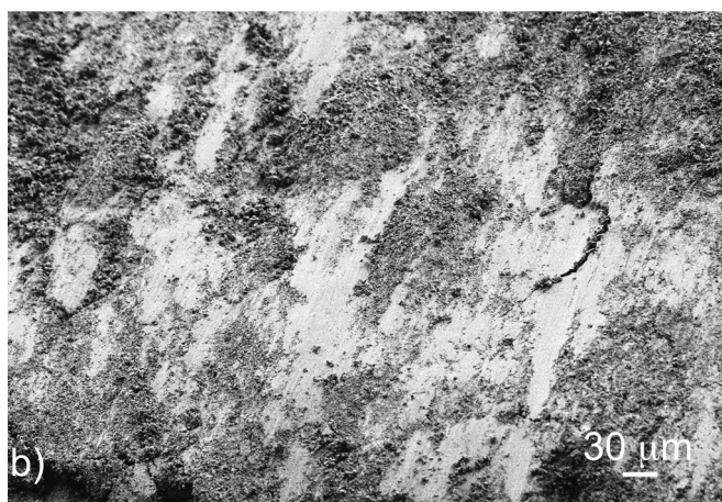
Fig. 13. The fracture surface of the Cr-doped test bar crept at 1000 °C to 17.1% strain. (a) Below the surface of the gauge length. (b) Close to the centre of the test bar.
