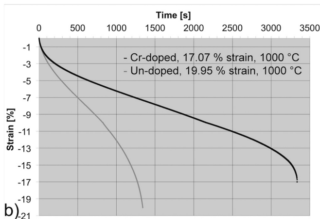
Fig. 7. Compressive creep curves registered during creep testing at 1000 °C. The un-doped material was deformed to 9.9% (a) and 19.9% (b) strain, and the Cr-doped material to 9.9% (a) and 17.1% (b) strain.
