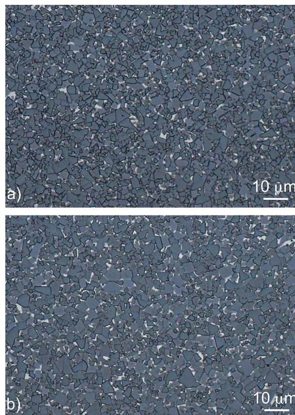
Fig. 4. Optical micrographs of etched surfaces from the as-sintered un-doped (a) and Cr-doped (b) materials. The Co-rich binder phase appears with bright contrast.
