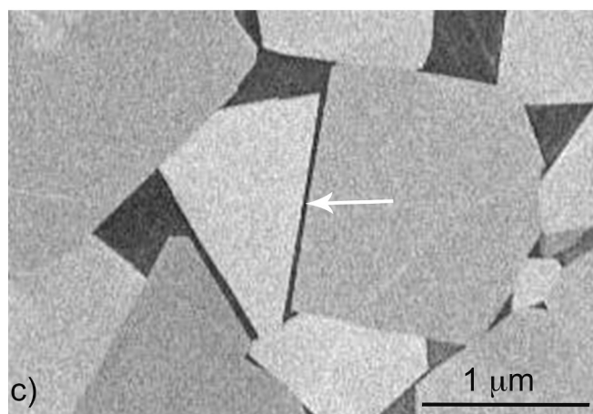
Fig. 15. (a) The general microstructure of the un-doped test bar crept at 1100 °C to 8.7% strain. The WC grains appear with bright contrast, the binder phase with dark, and the cavities (arrowed) with black contrast. (b) and (c) Higher magnification details showing Co-rich films at WC grain boundaries. Some WC grain surfaces, arrowed in (b), have a saw-tooth like appearance. Other WC grain boundaries contain a thin binder phase lamella, arrowed in (c). The WC grain surface arrowed in (b) has steps forming an angle of 120°.
