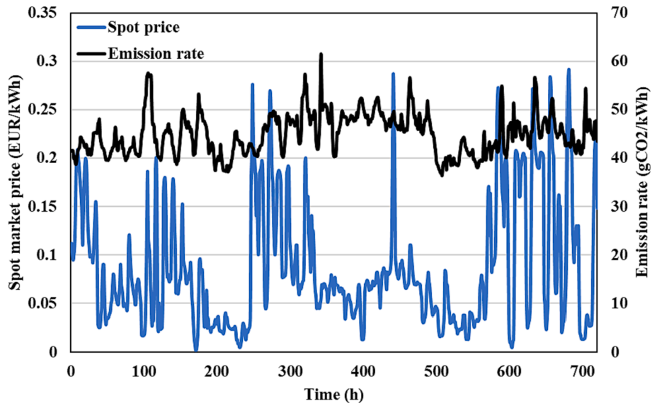
Fig. 5. Spot market price and CO 2 emission rate for the month of April 2022.
