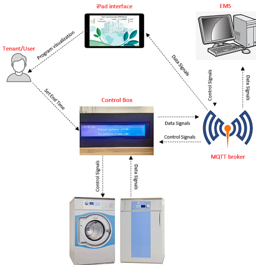
Fig. 3. Schematic diagram of the developed energy management system.
