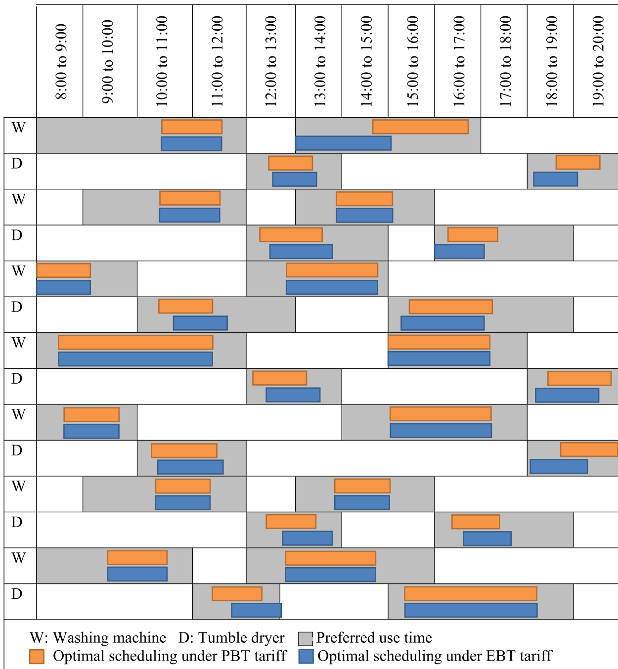
Fig. 8. The task profile and optimal service time during the study period.
