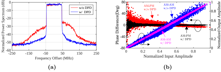
Figure 3.14: Modulated-signal measurement results of the three-stage Doherty PA prototype at 2.14 GHz. (a) Measured spectrum with and without DPD, (b) measured AM-AM and AM-PM characteristics with and without DPD, when using a 100-MHz 8.5-dB PAPR communication signal.
