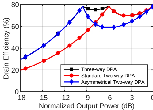
Figure 3.1: Drain efficiency versus normalized output power of different Doherty PA architectures: Standard two-way, asymmetrical two-way (N-way), and three-stage.
