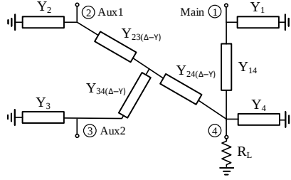
Figure 3.11: Simplified combiner network after tuning of z_{44} and \Delta - Y transformation.
