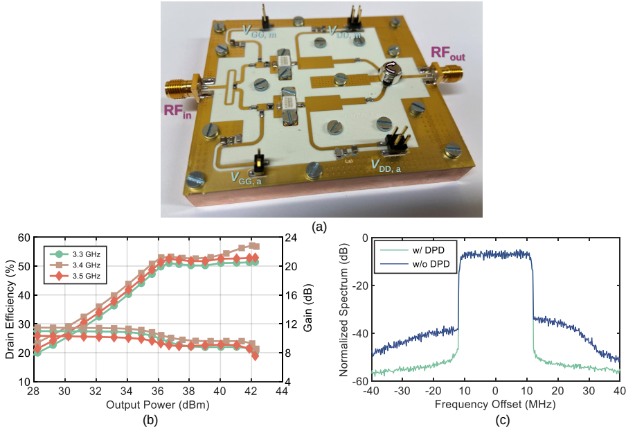
Figure 4.10: (a) Photo of the CLMA prototype circuit. (b) Measured drain efficiency of the CLMA prototype circuit versus the output power from 3.3 to 3.5 GHz and (c) Normalized spectrum of the prototype circuit when applying a 20-MHz 7-dB PAPR OFDM signal at 3.4 GHz, before and after applying DPD. [Paper E]
