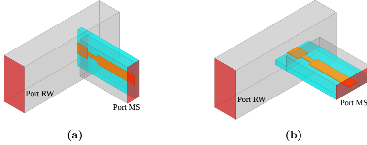
Figure 2.7: (a) broadside E-plane transition from microstrip to waveguide, (b) longitudinal H-plane transition from microstrip to waveguide [54].
