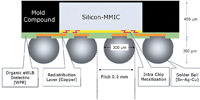
Figure 2.2: Cross-sectional view of an eWLB package [46].
