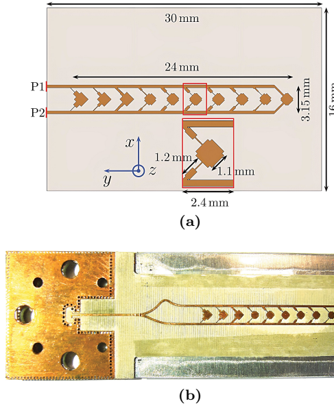
Figure 3.5: Configuration of the proposed patch array (a) dual linearly polarized and (b) left hand circularly polarized [11].
