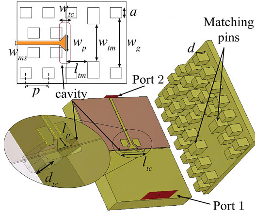
Figure 2.12: Configuration of the proposed microstrip-to-waveguide inline transition [37].
