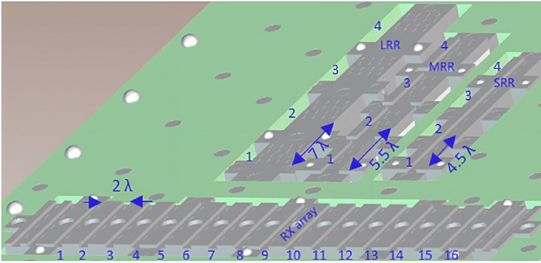
Figure 3.3: Simultaneous multi-mode automotive imaging radar system using waveguide slot arrays. [53].
